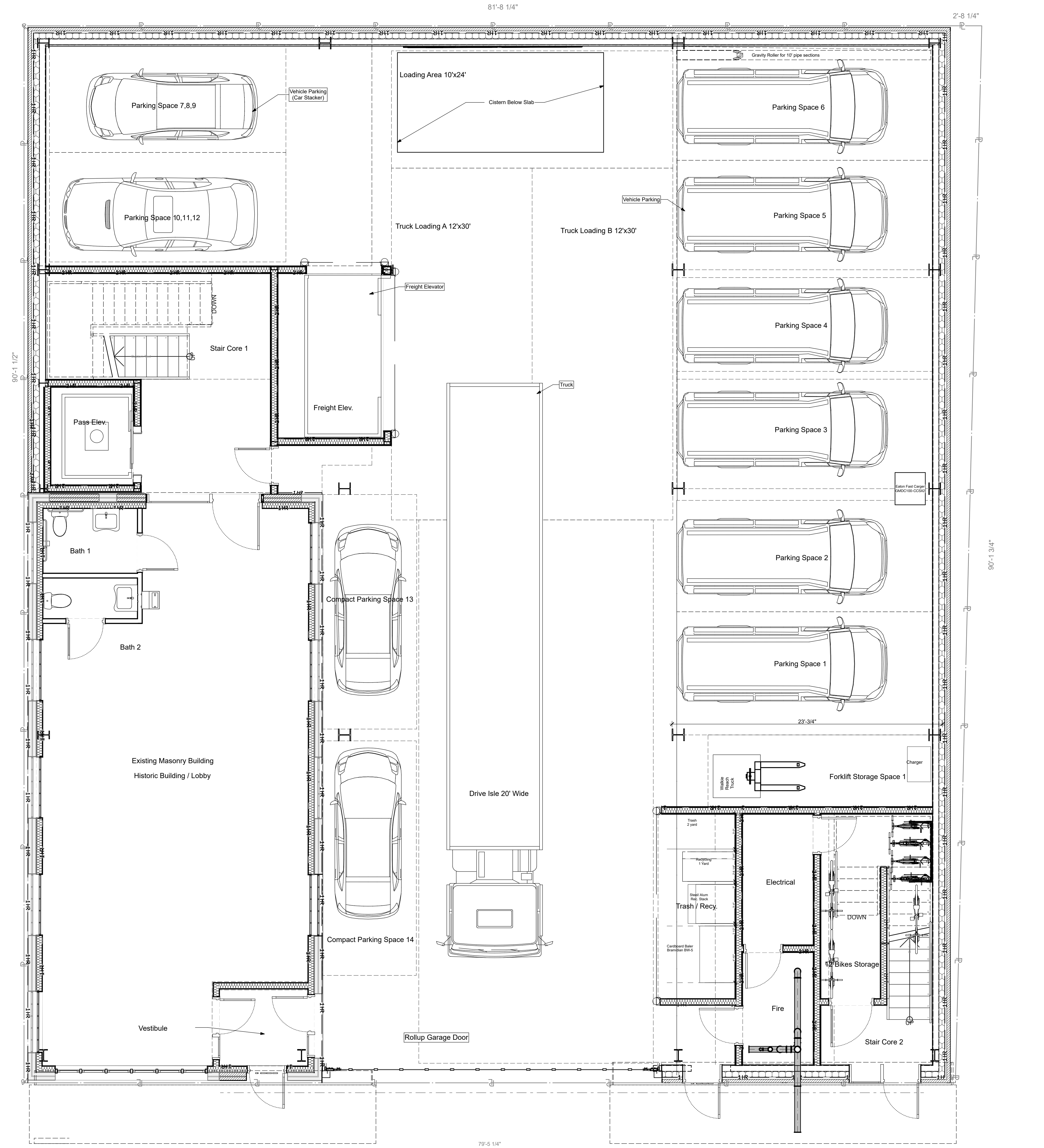
1 First Floor Plan BZA100 SCALE: 1/4" = 1'-0"
