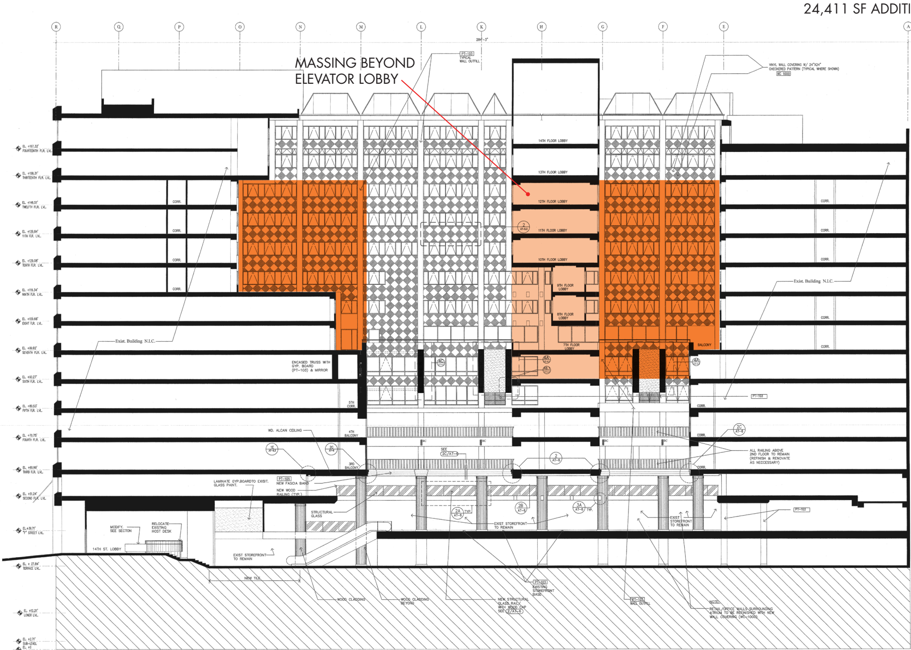
SECTION LOOKING NORTH (A-A)
