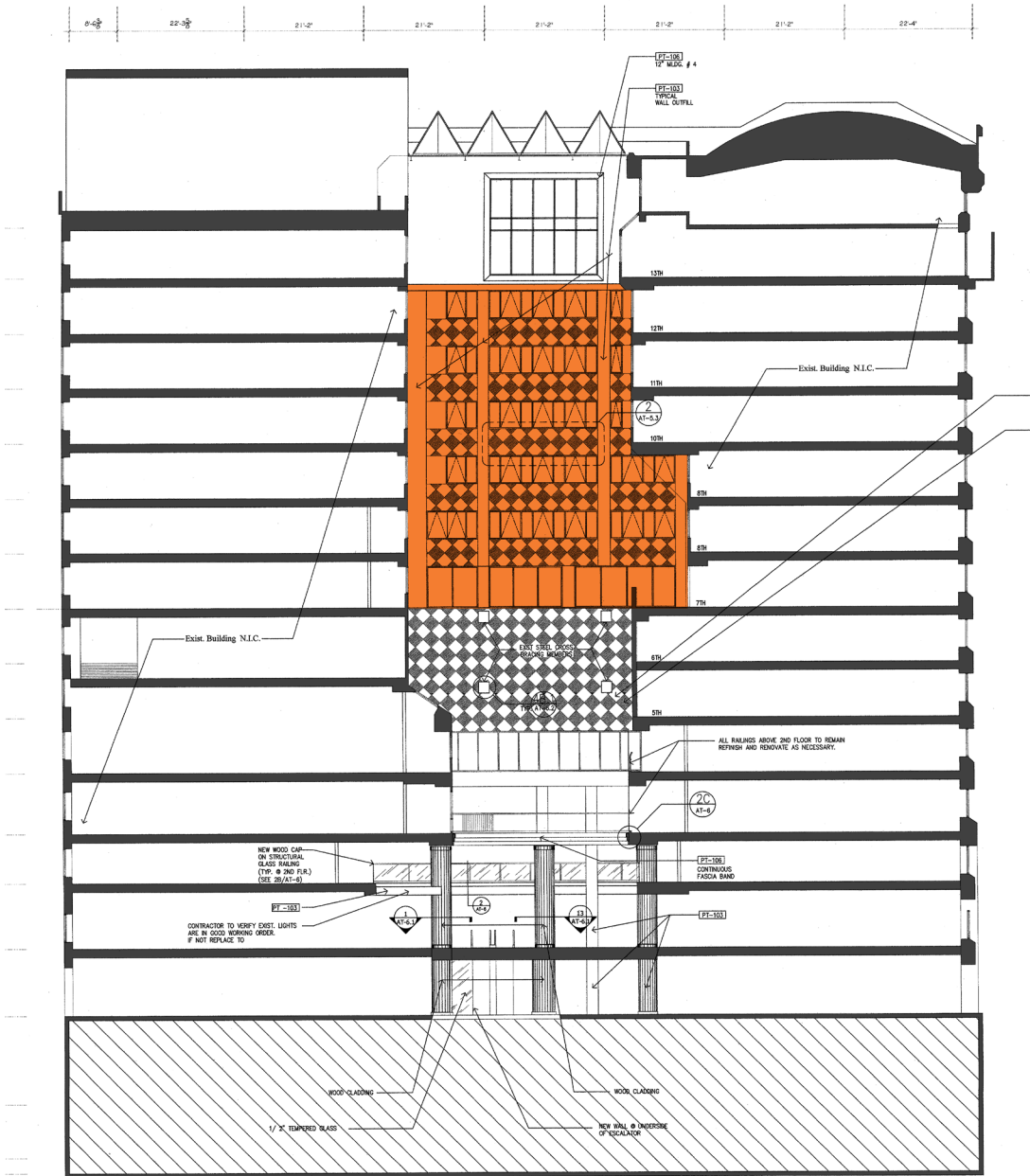
SECTION LOOKING WEST (B-B)
