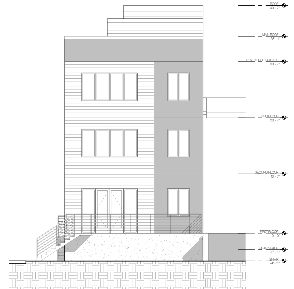
③ SOUTH (REAR) ELEVATION
