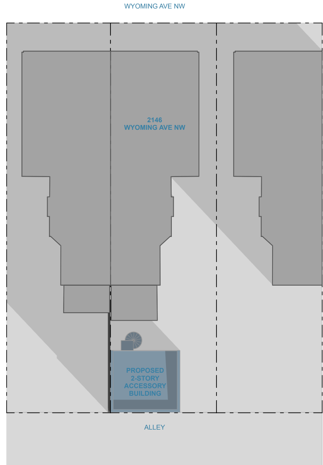
WINTER 9AM PROPOSED
