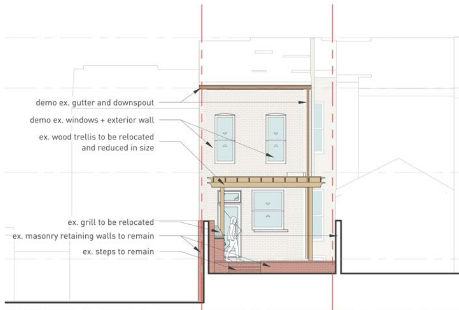
existing elevation
