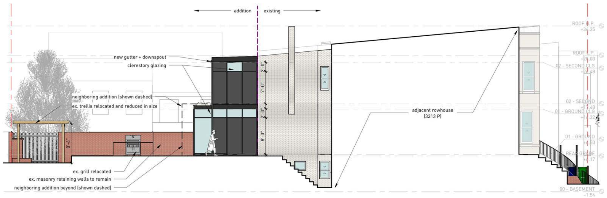
proposed elevation
