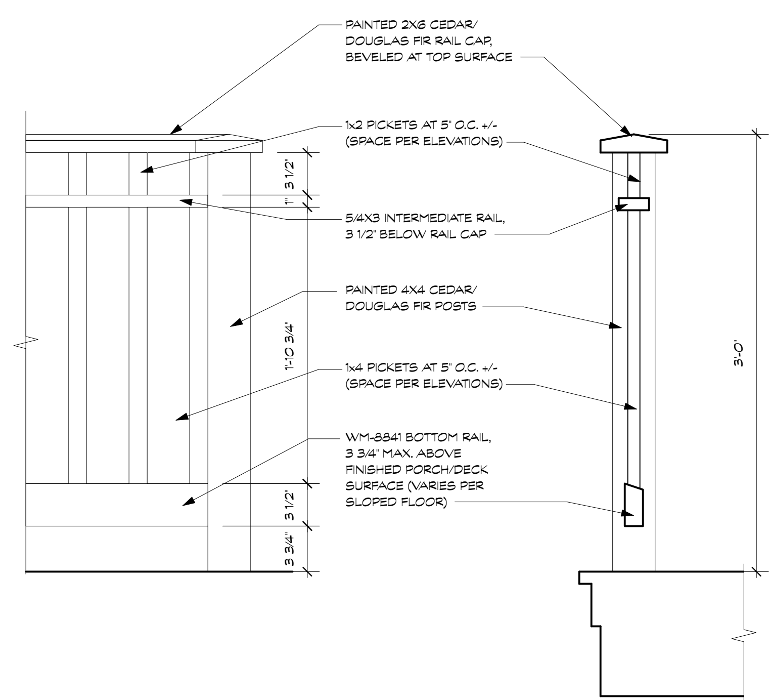
A PORCH RAILING DETAIL Scale: 1 1/2" = 1'-0"
