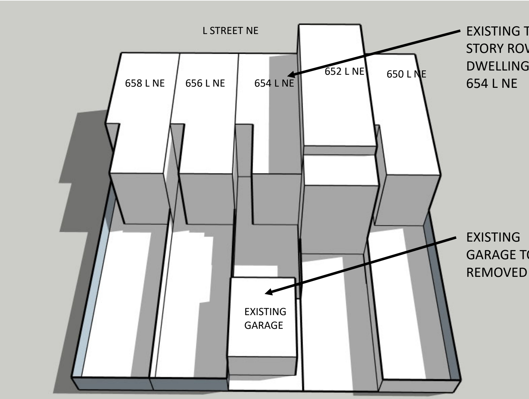
June 21 st 3:00 PM EXISTING
