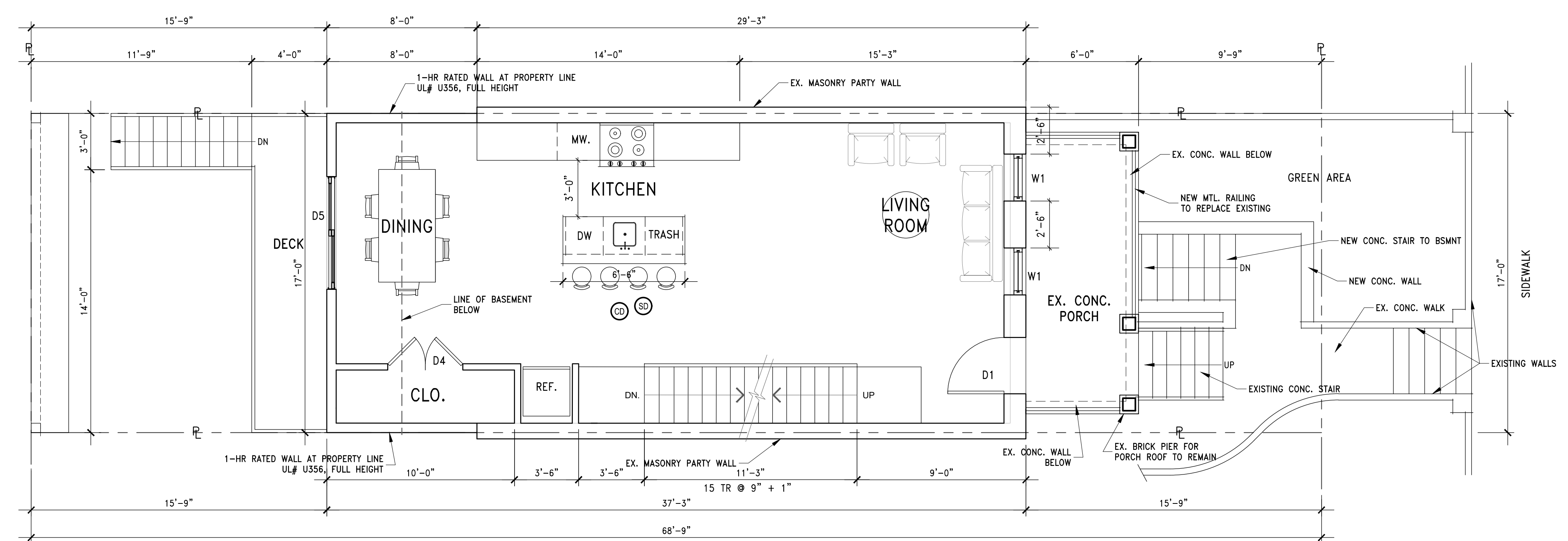
2 PROPOSED FIRST FLOOR PLAN A0001 SCALE: 1/4"=1'-0"
