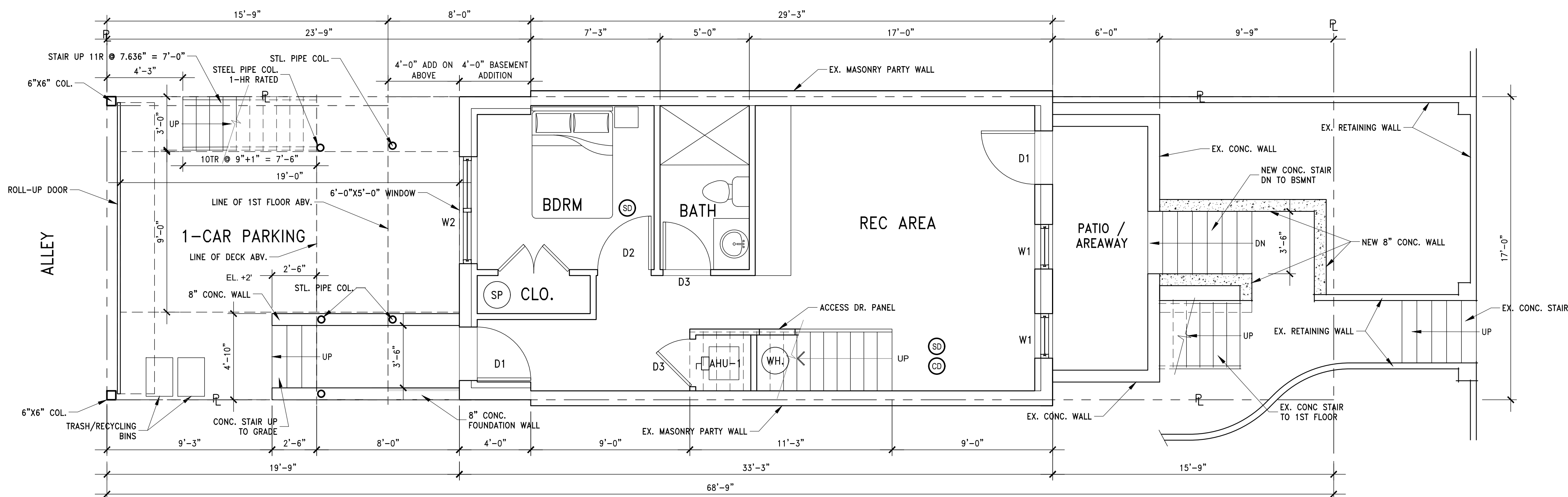
1 PROPOSED BASEMENT PLAN A0001 SCALE: 1/4"=1'-0"
