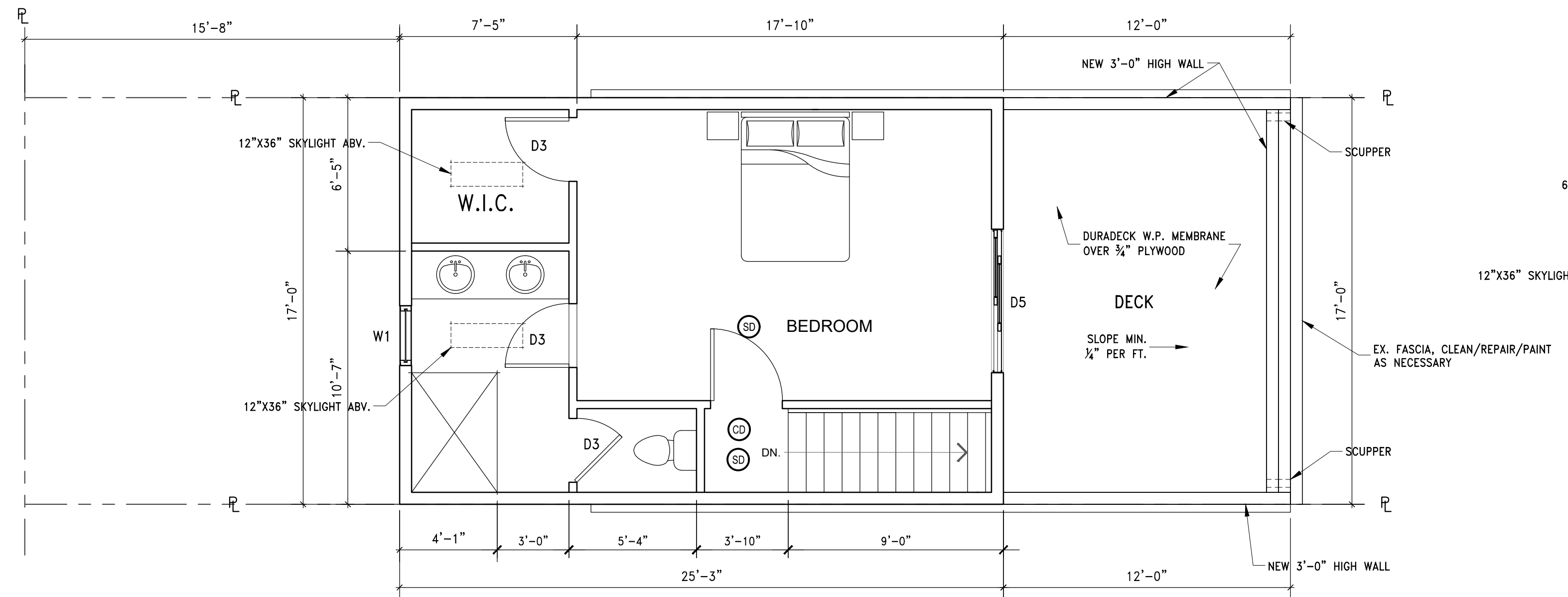
2 PROPOSED THIRD FLOOR PLAN A0002 SCALE: 1/4"=1'-0"
