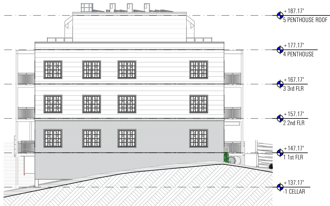
2 East Elevation SCALE: 1/16" = 1'-0"
