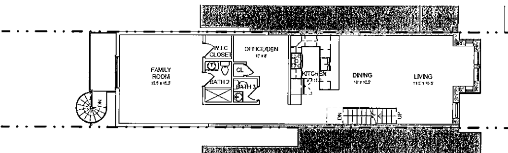
PROPOSED SECOND FLOOR
