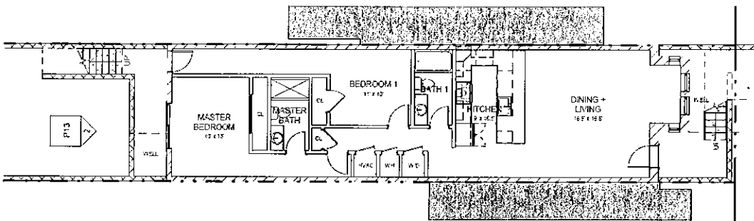
PROPOSED CELLAR
