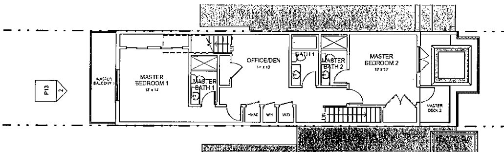
PROPOSED THIRD FLOOR
