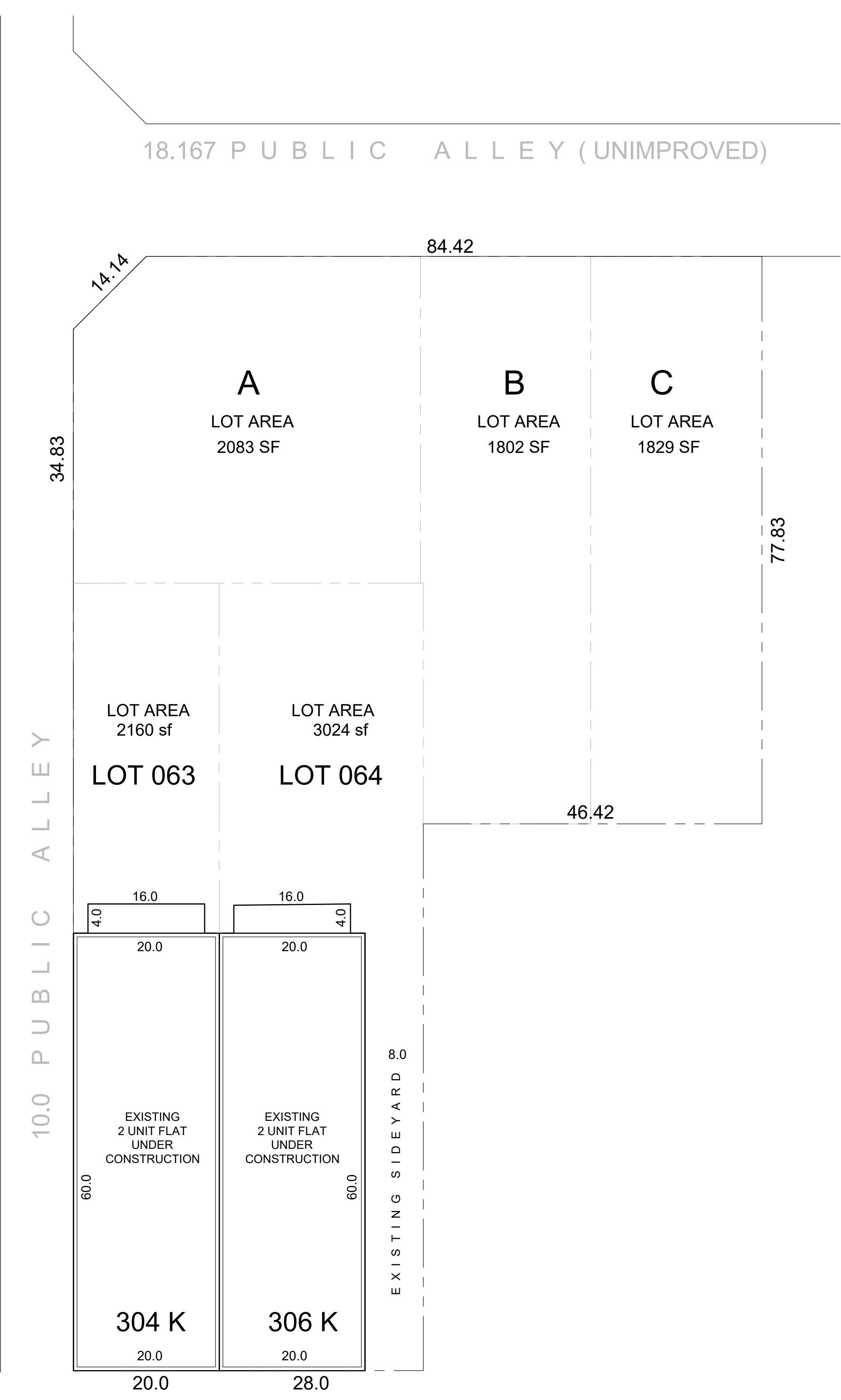
PROPOSED SUBDIVISION
