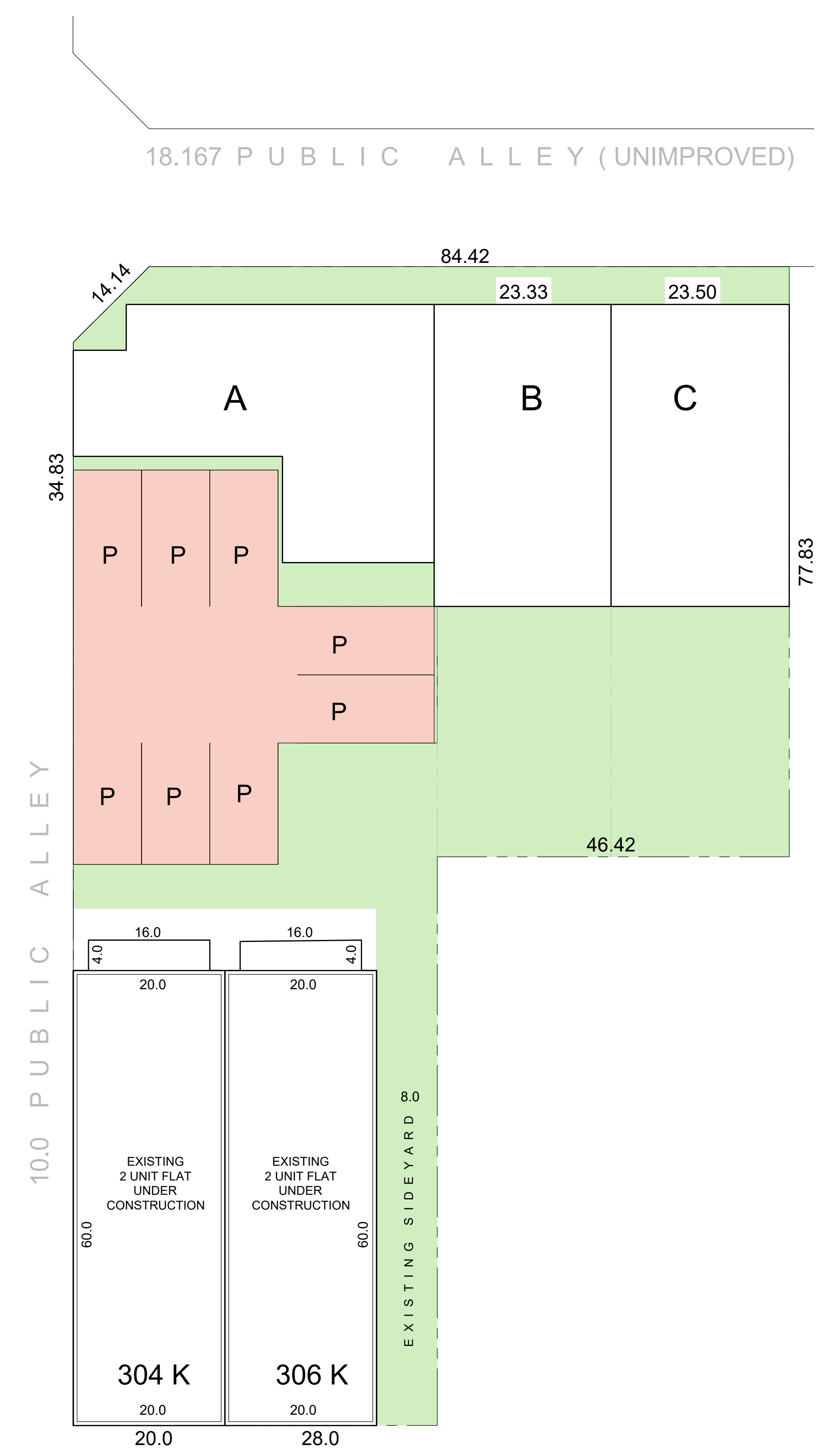
PROPOSED IMPROVEMENTS
