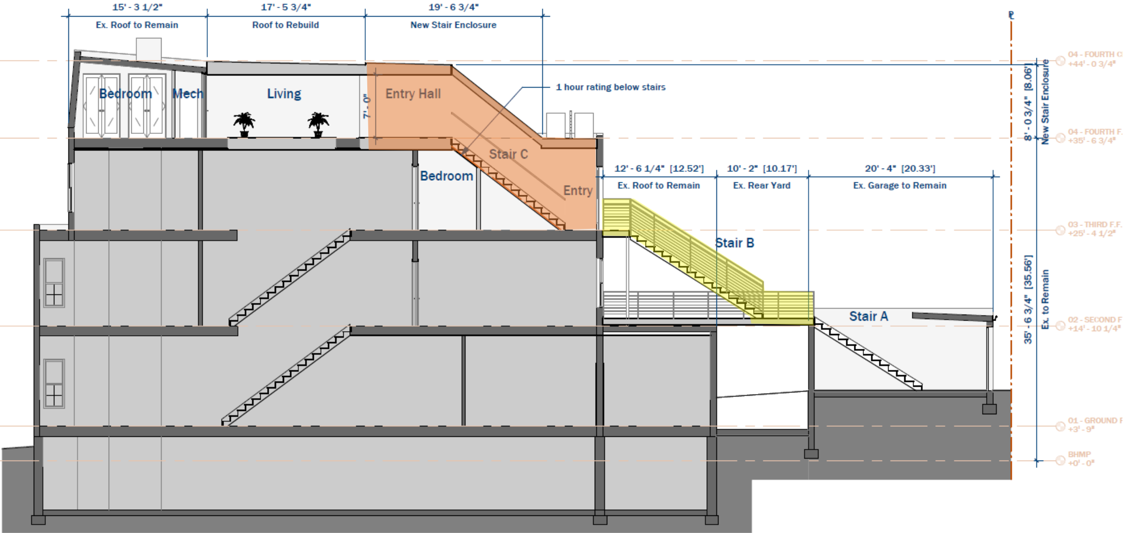
Building Section
