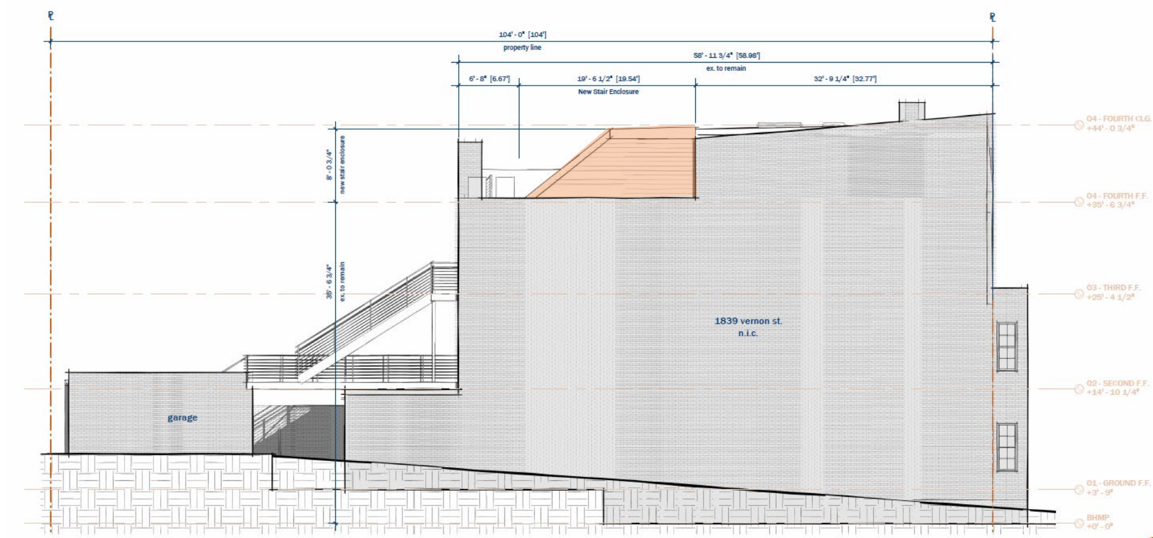
Building Elevation - West
