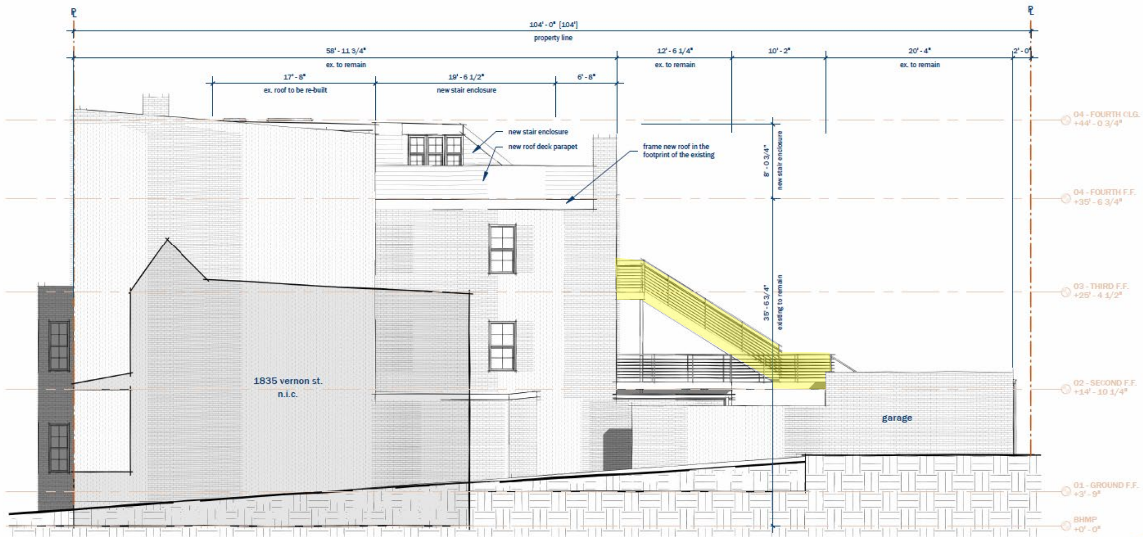
Building Elevation - East
