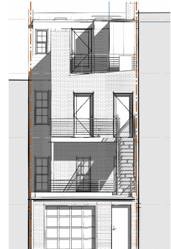
Proposed Elevation
