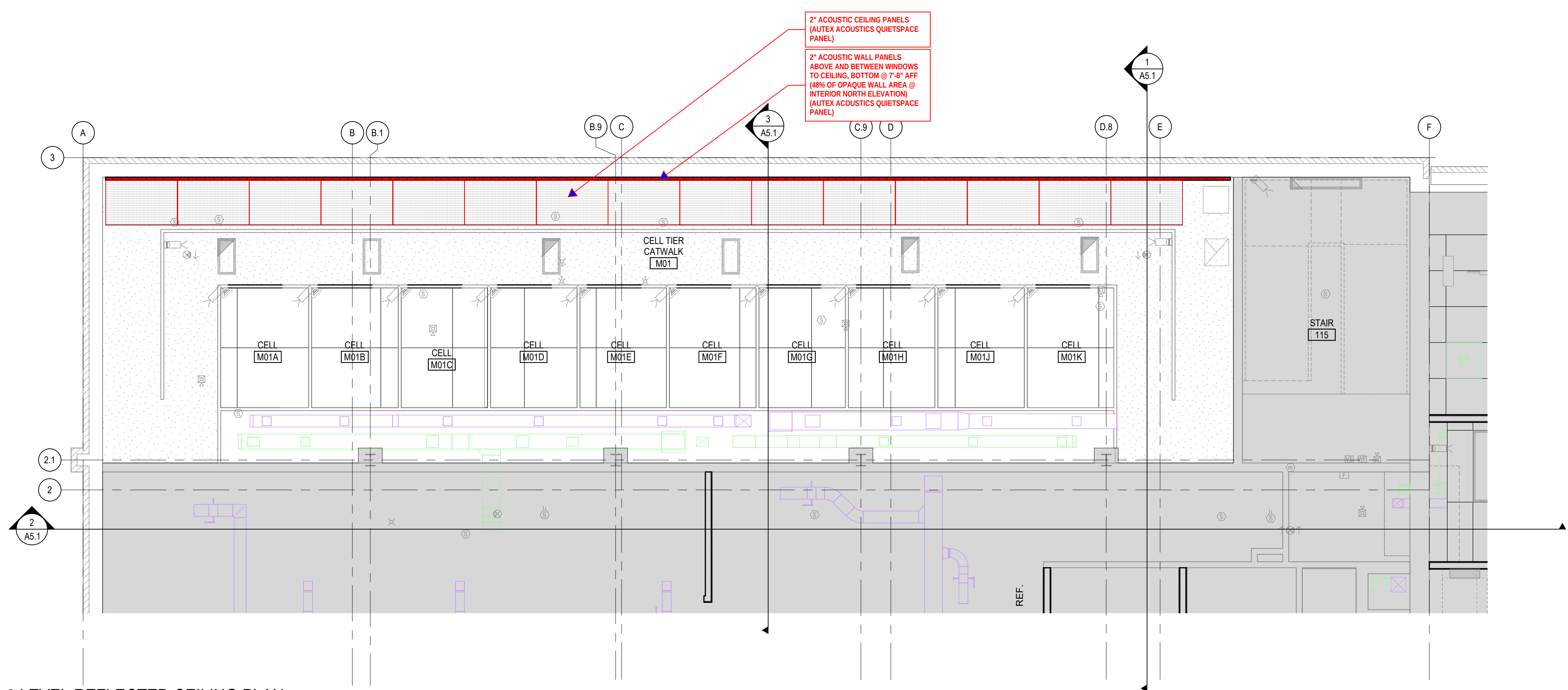
2 TIER 2 LEVEL REFLECTED CEILING PLAN A32 SCALE: 1/4" = 1'-0"
