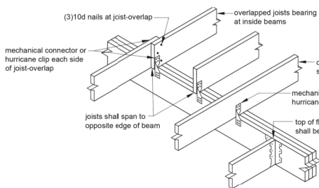
FIGURE 10: JOIST-TO-BEAM CONNECTION
