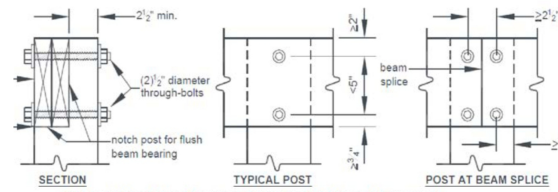
FIGURE 18: NOTCHED 6x6 POST-TO-BEAM CONNECTION
