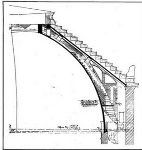
Longitudinal Section, Showing Method of Construction
