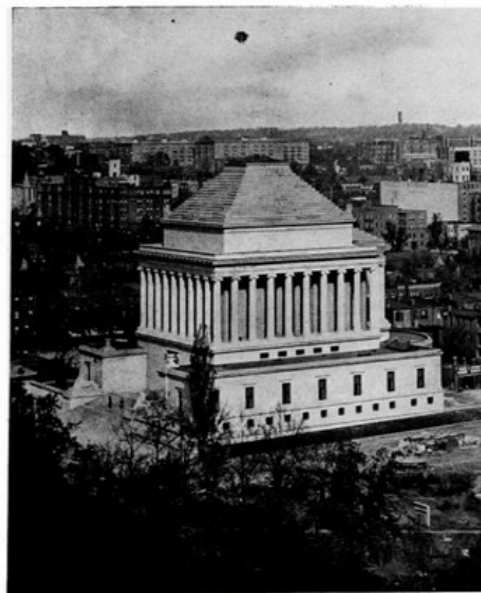
View of Building, Showing Solid Limestone Roof
