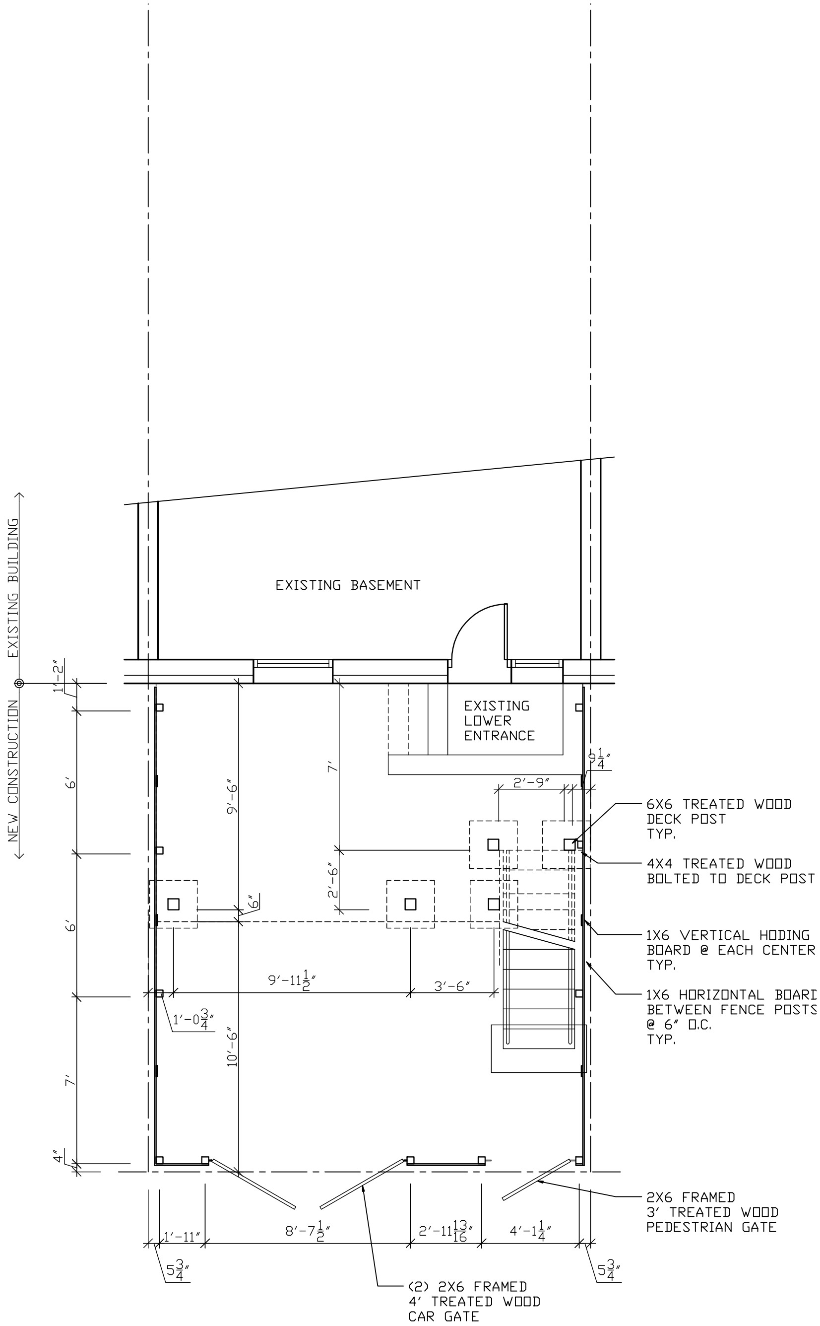
1 S-02 GROUND LEVEL PLAN SCALE: 1/4"=1'-0"
