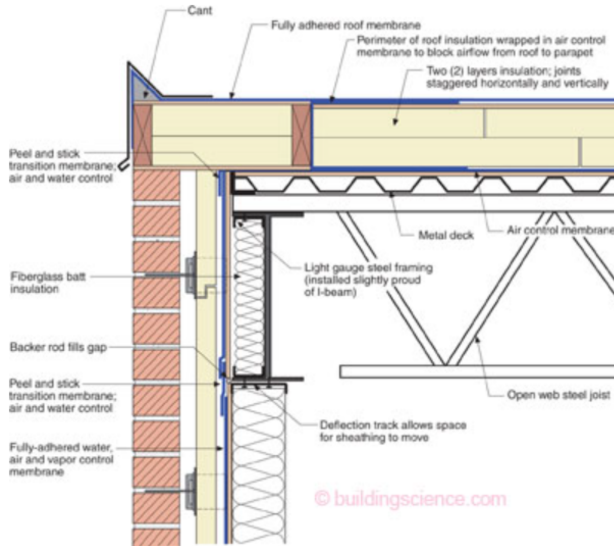
Figure 15: The Cantilevered Mini Parapet —Notice that air control layer continuity is achieved by wrapping the membrane over the building corner and then constructing the cantilevered portion of the parapet over the top of this air seal.
