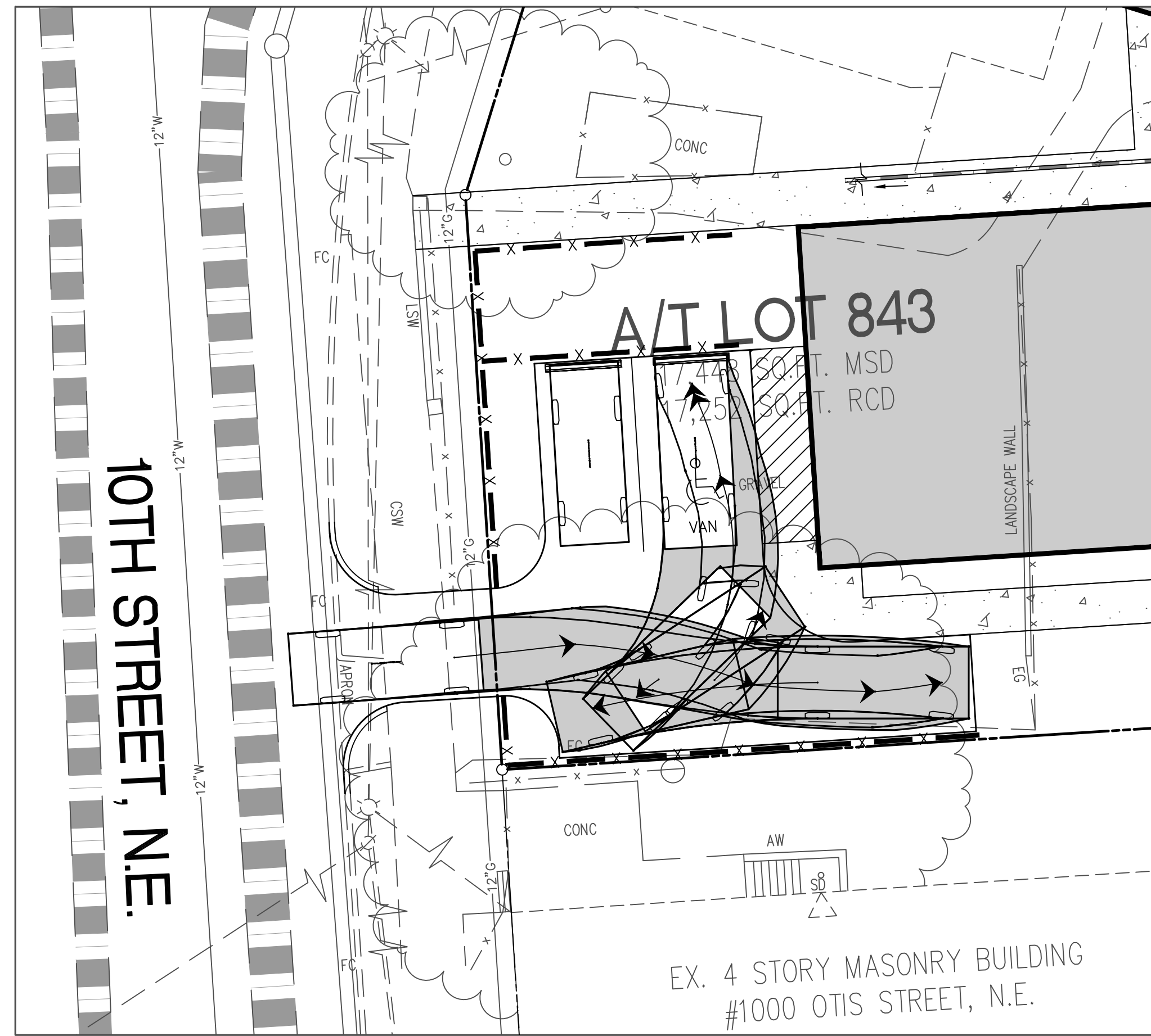
WHEELCHAIR VAN SPACE 2 - ENTER
