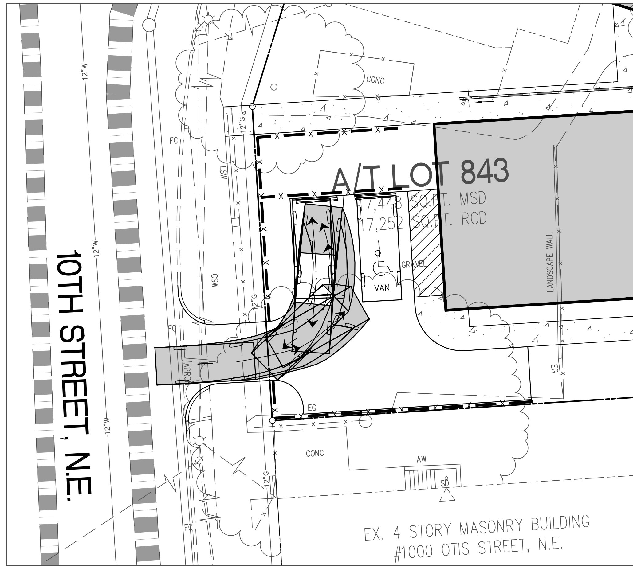
PASSENGER CAR SPACE 1 - ENTER
