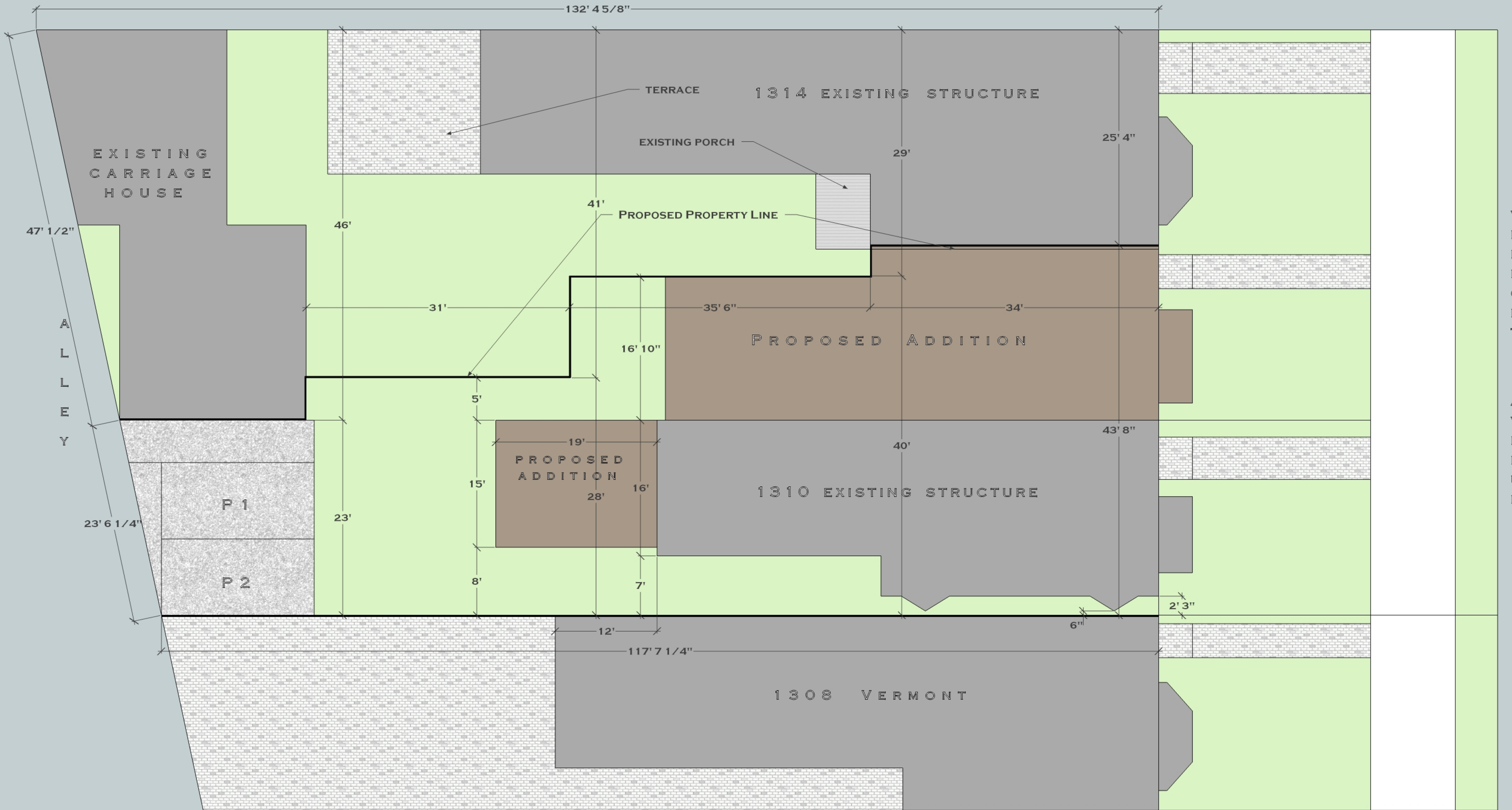
PROPOSED SITE PLAN
