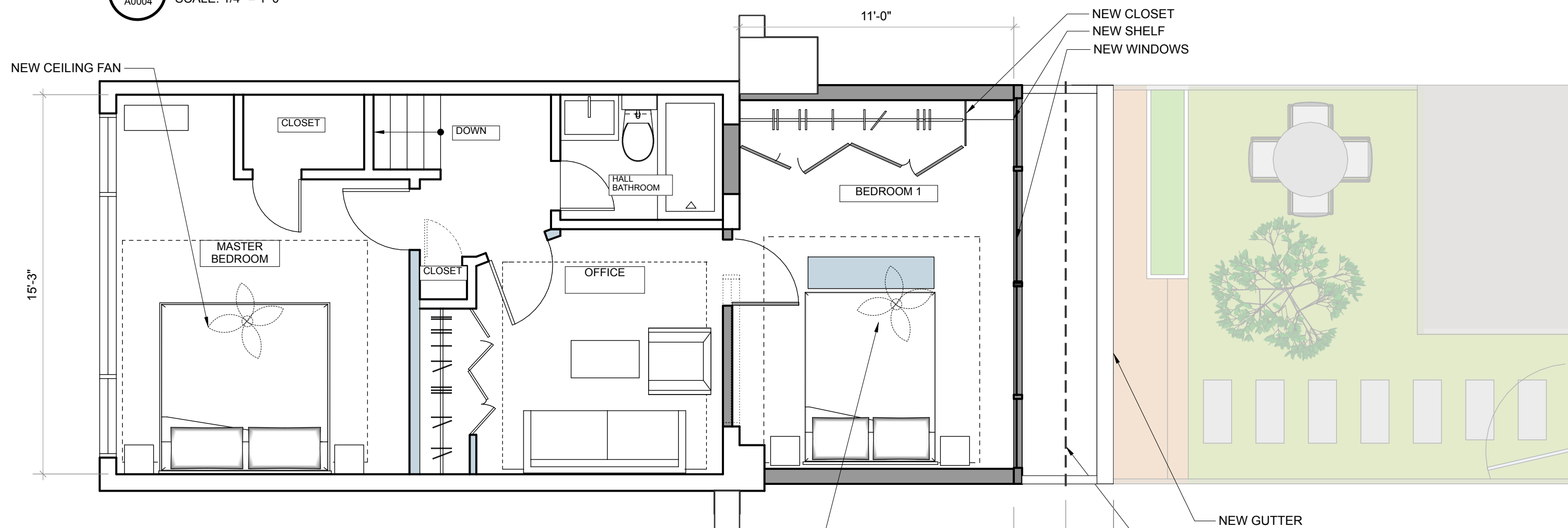
3 THIRD FLOOR - PROPOSED A0004 SCALE: 1/4" = 1'-0"
