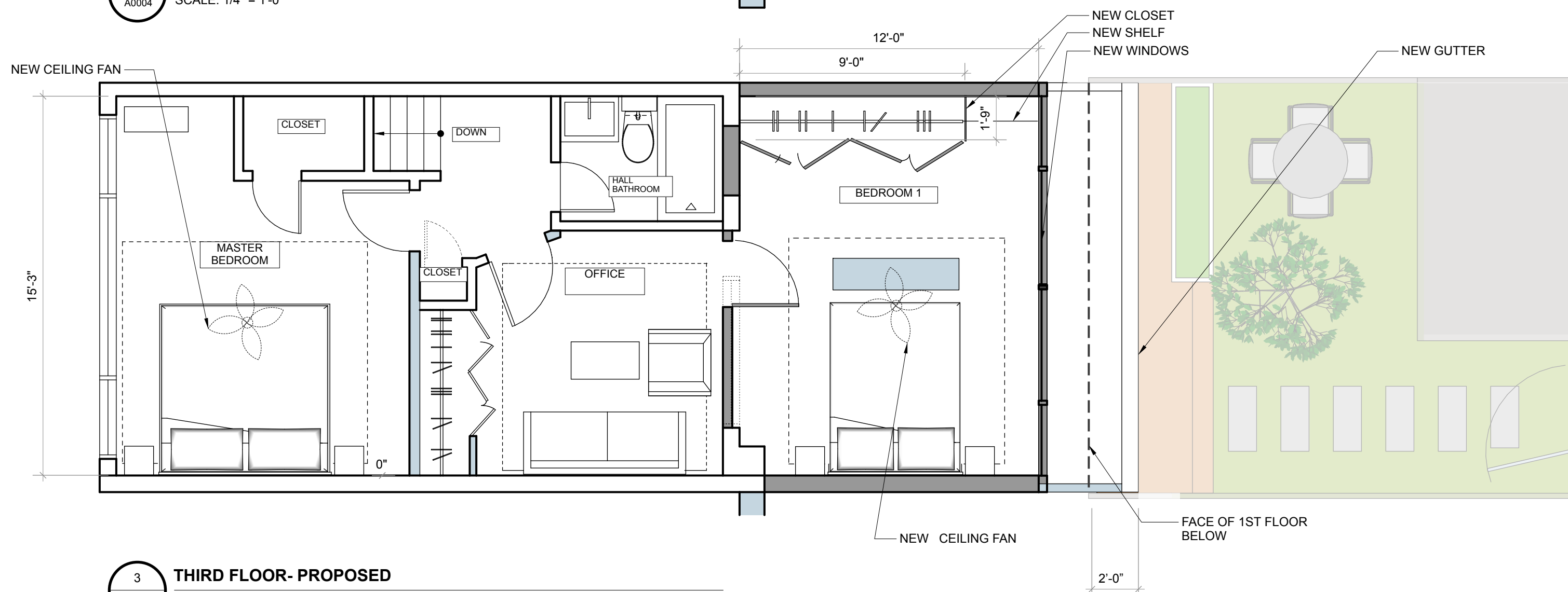
2 SECOND FLOOR - PROPOSED A0004 SCALE: 1/4" = 1'-0"
