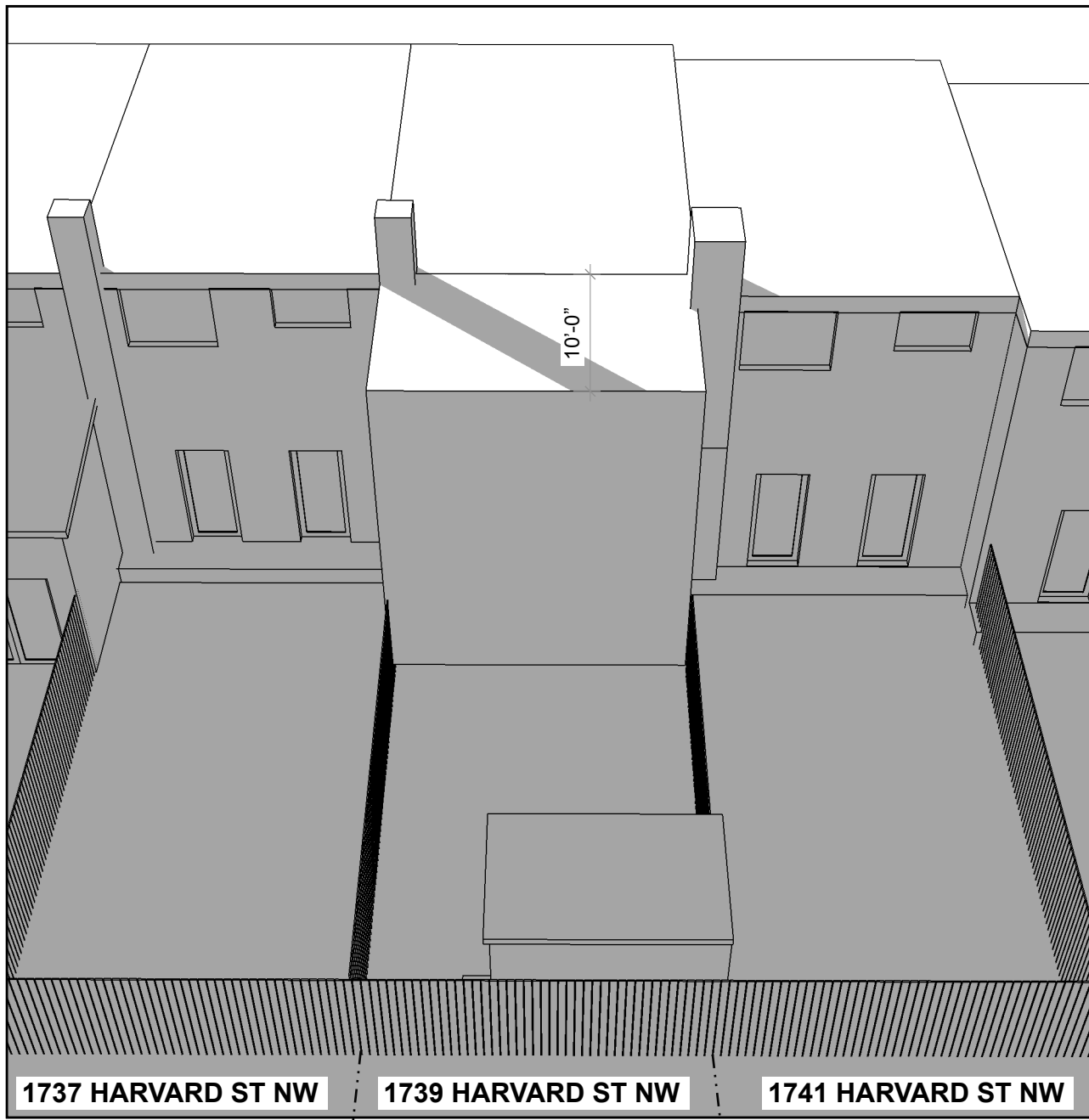
1 10'-0" ADDITION SHADOW STUDY - DEC 21 @ 9AM A0013 NTS
