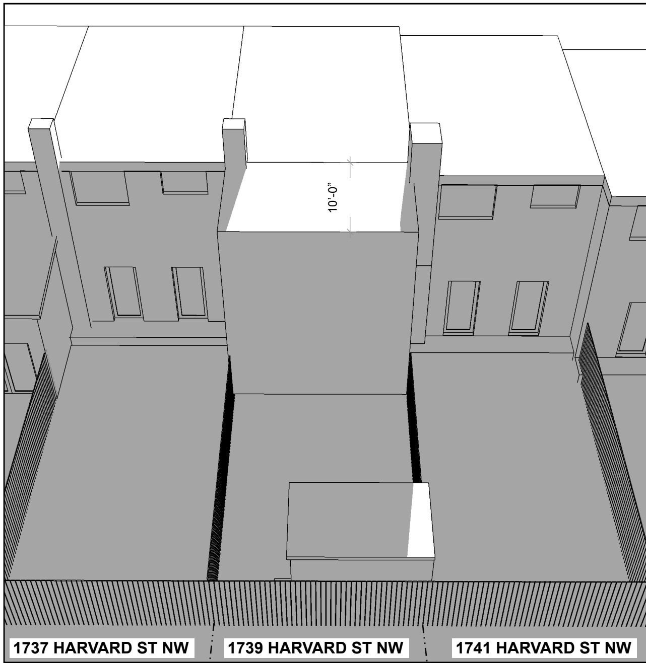
4 10'-0" ADDITION SHADOW STUDY - DEC 21 @ 1PM A0013 NTS
