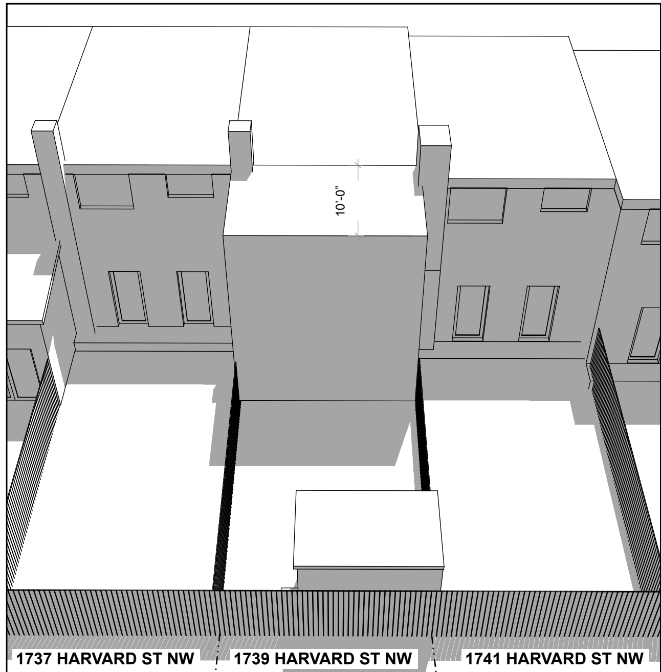
4 10'-0" ADDITION SHADOW STUDY - JUNE 21 @ 1PM A0009 NTS
