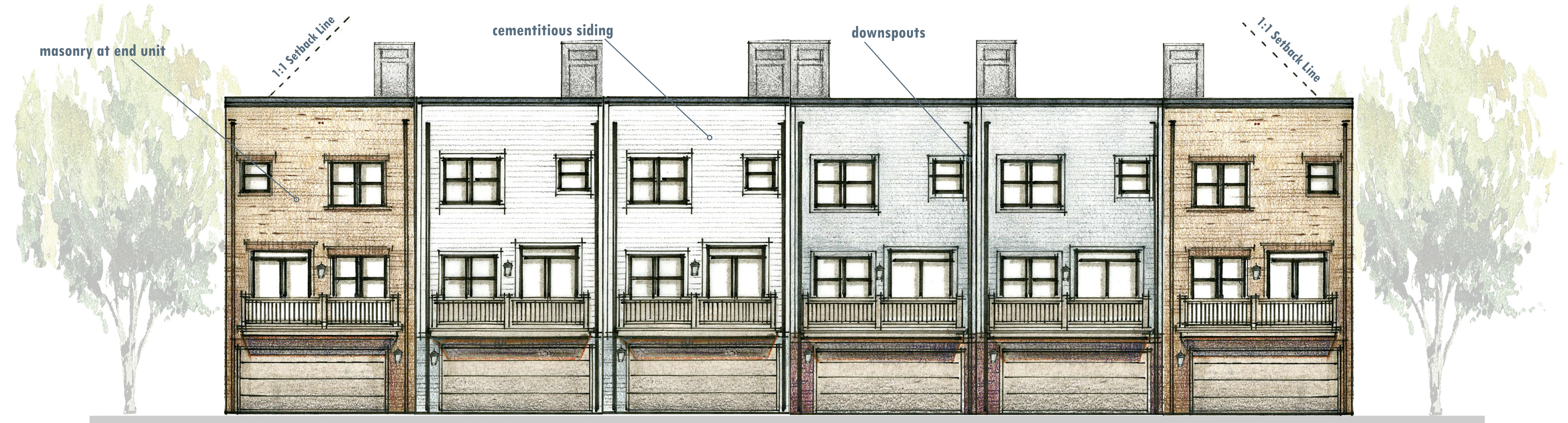
Rear Elevations
