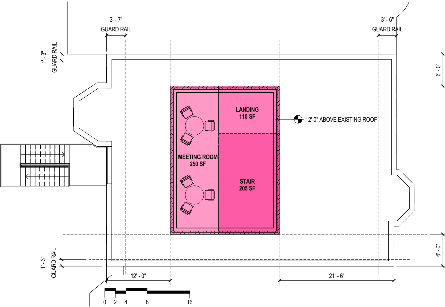
BY RIGHT PENTHOUSE
