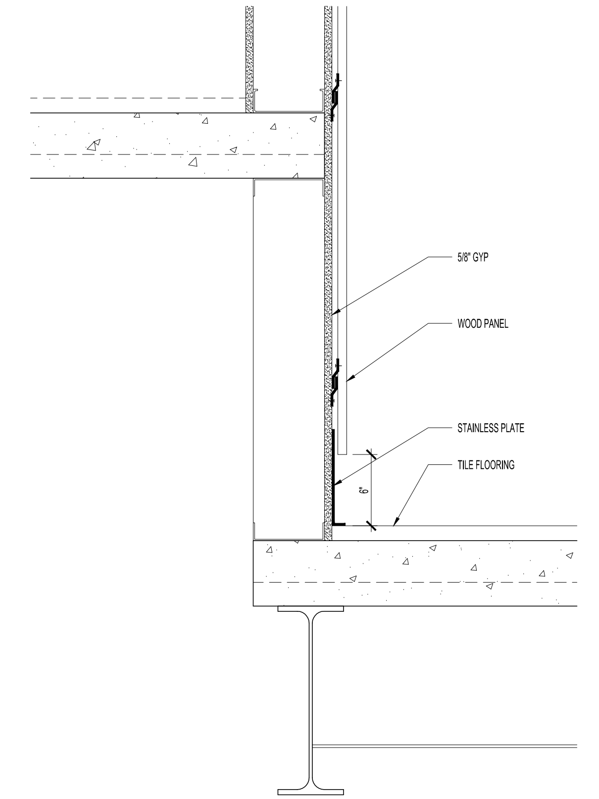
7 SLAB BREAK DETAIL
