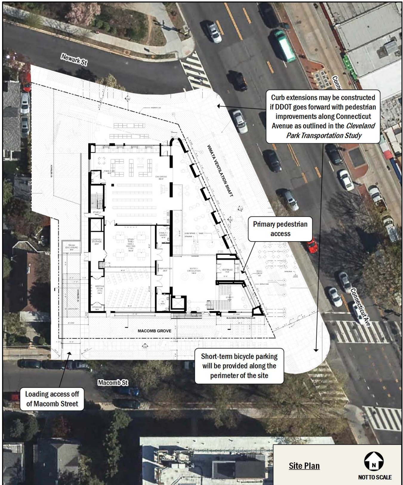
Figure 4: Site Plan
