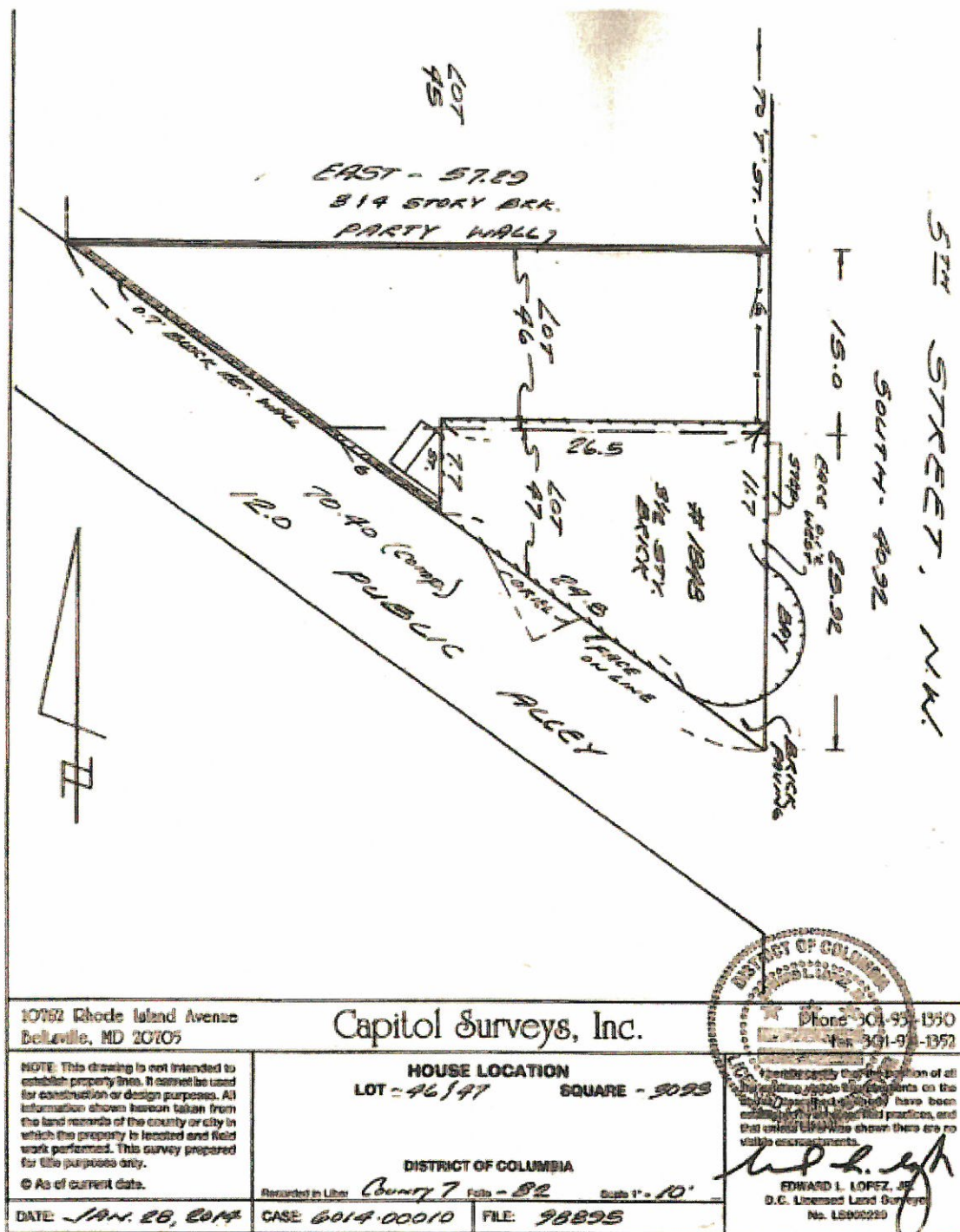
Figure 3. Recent Survey of Lots 47 and 46.
