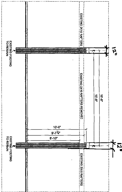
1 EXISTING GARAGE SECTION SCALE: 3/8" = 1'-0" 24X36 LAYOUT
