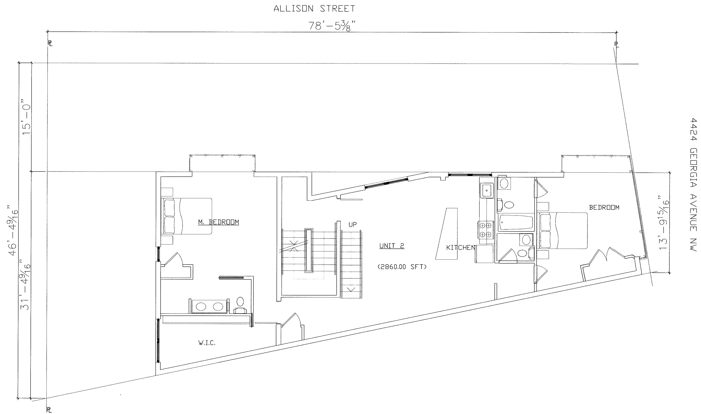
6 PLAN: FIFTH FLOOR 1/8" = 1'-0"
