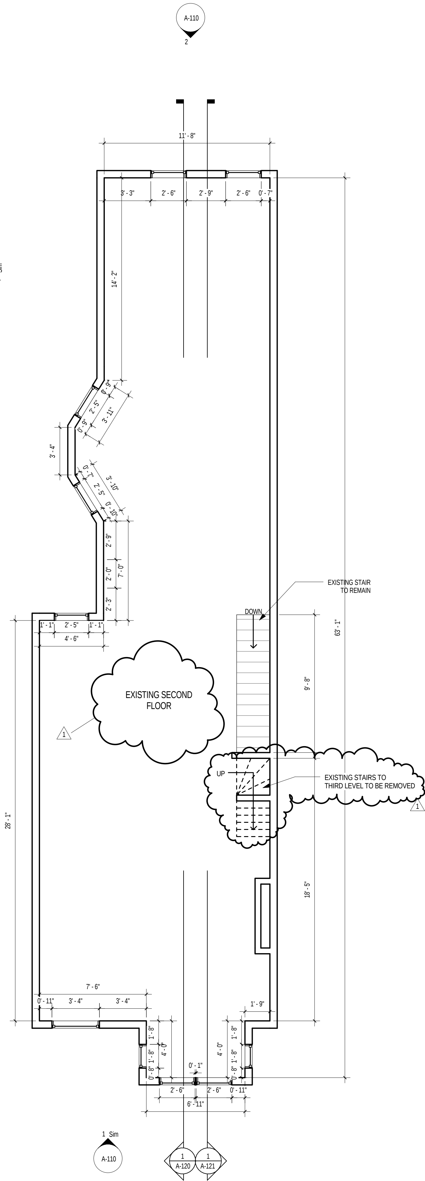
3 EX. LEVEL 2 1/4" = 1'-0"
