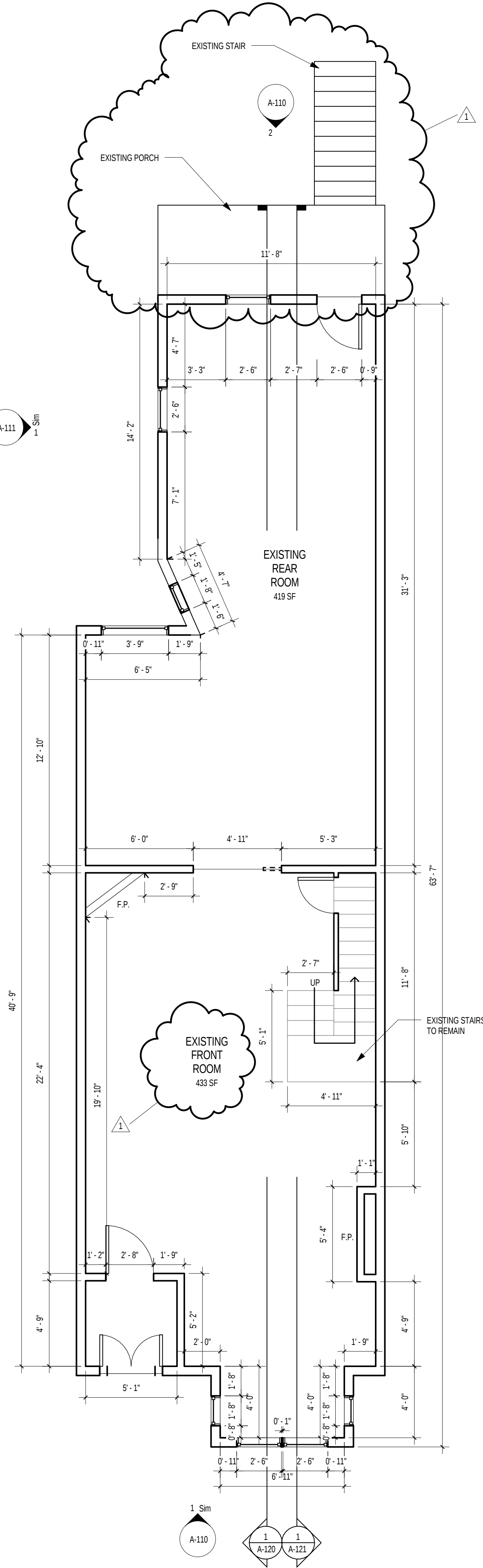
2 EX. LEVEL 1 1/4" = 1'-0"
