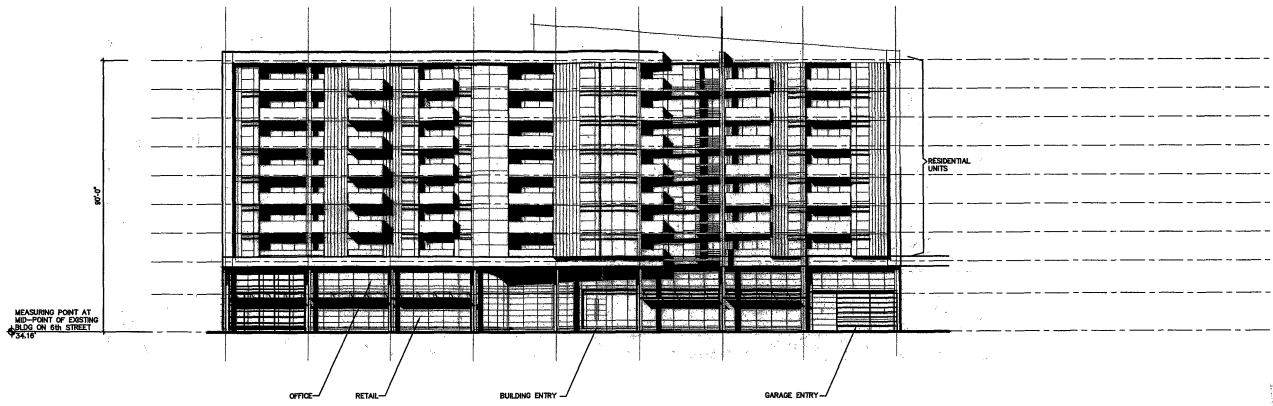
1 NORTH ELEVATION 1/16" = 1'-0" 306_P3.dwg
