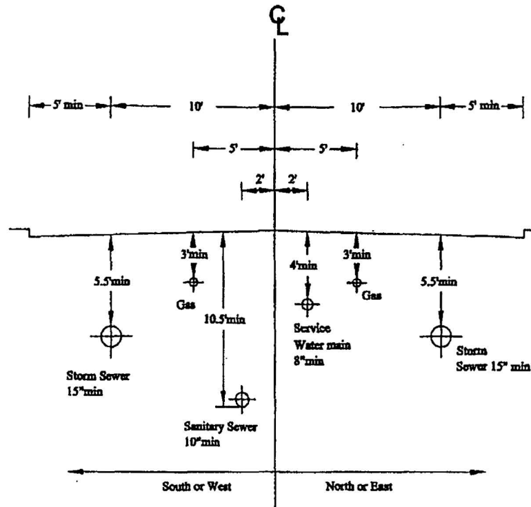
Figure 3-B3-1 Typical Location of Underground Utilities Streets with Single Water and Sewer Services
