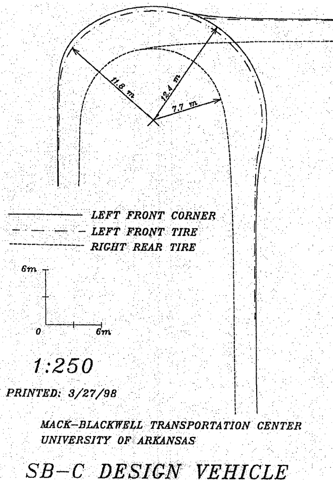
FIGURE 11 Recommended Metric Type "C" School Bus Turning Template
