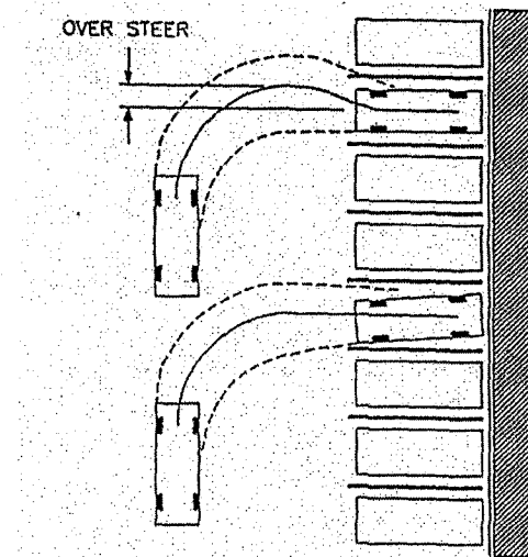
FIGURE 5 Example of Oversteer
