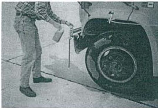
FIGURE 2 Burettes on Bus Body and Tire Water Spraying Apparatus
