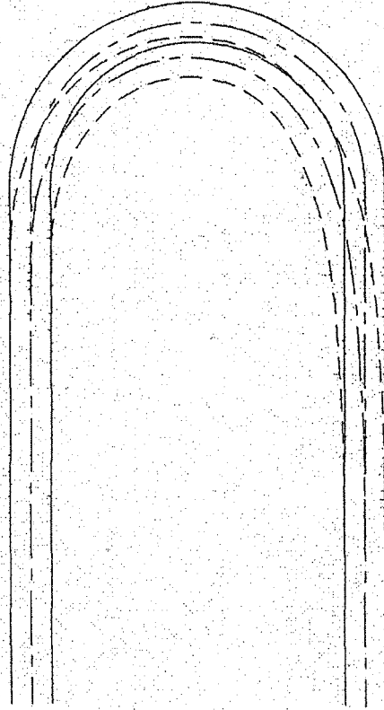
FIGURE 9 Airplane Graphical Method Type "D" School Bus Turn Path
