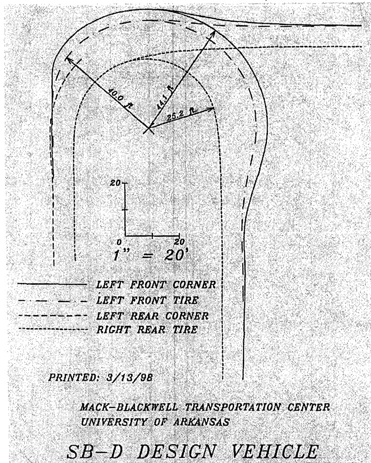
FIGURE 12 Recommended Type "D" School Bus Turning Template
