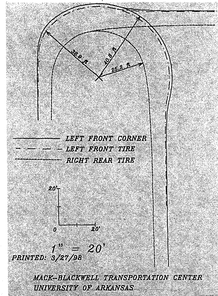
FIGURE 10 Recommended Type "C" School Bus Turning Template
