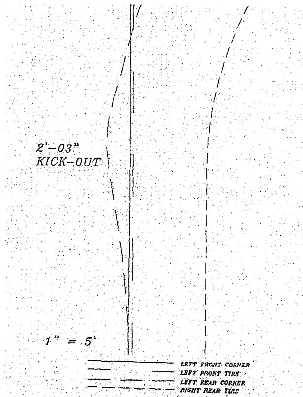
FIGURE 4 Rear Body "Kick-Out" Effect
