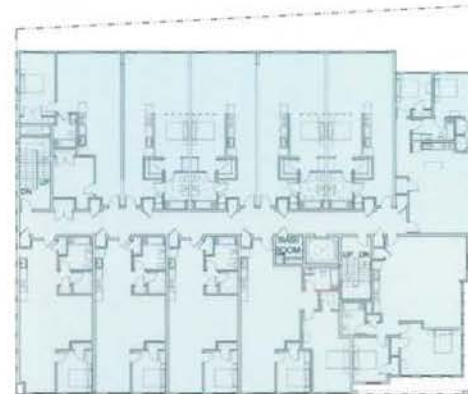
SECOND FLOOR PLAN SCALE: 1/16" = 1'-0"
