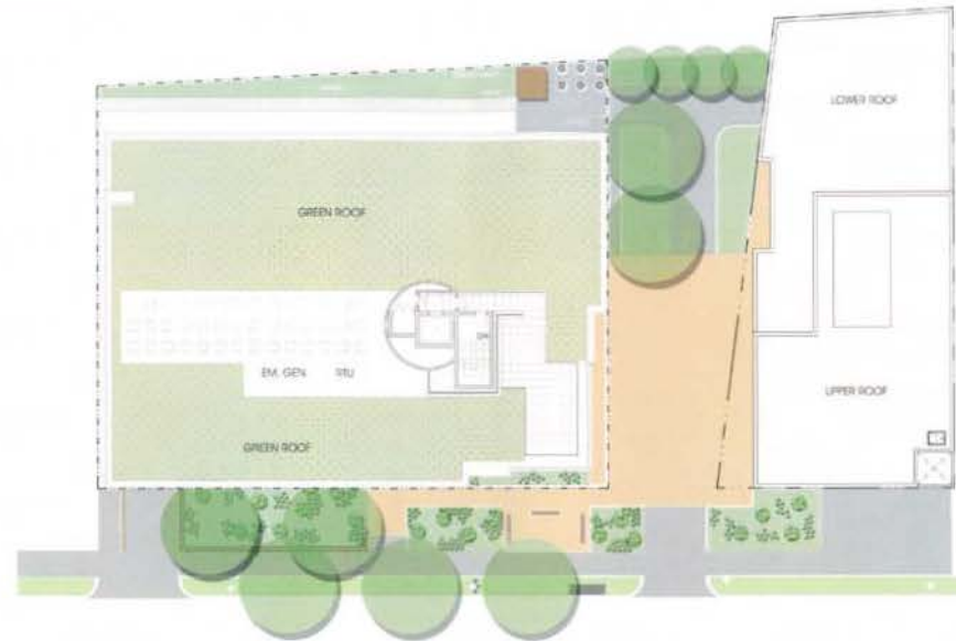
ROOF PLAN SCALE 1/16" = 1'-0"
