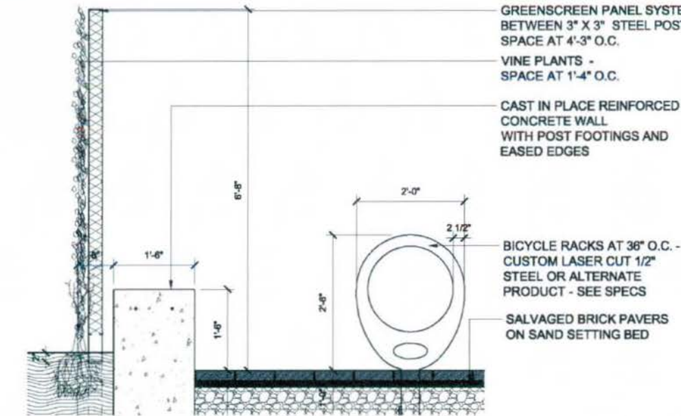
GREEN SCREEN / BICYCLE RACK 3/4" = 1'-0"
