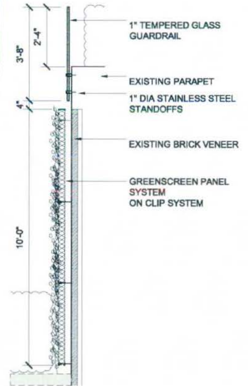
GREEN SCREEN AT ENTRY 1/2" = 1'-0"
