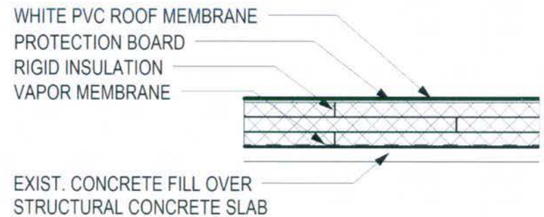
WHITE PVC MEMBRANE ROOF DETAIL
