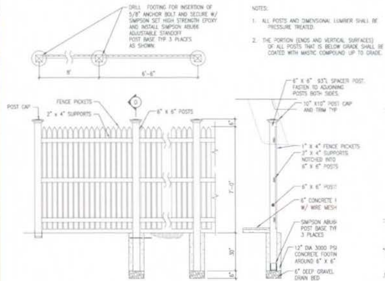
PREVIOUS OPTION TRASH ENCLOSURE DETAIL SCALE: 1/8" = 1'-0"
