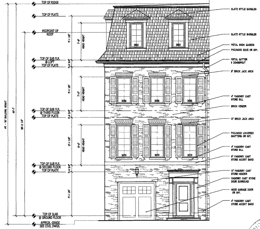
UNIT D FRONT ELEV. #2
