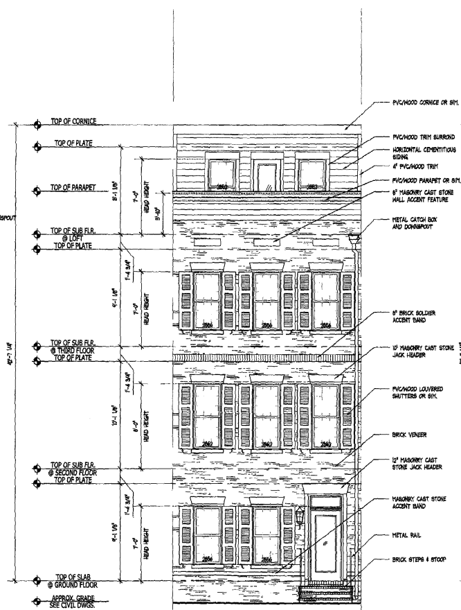
UNIT B FRONT ELEV. #2
