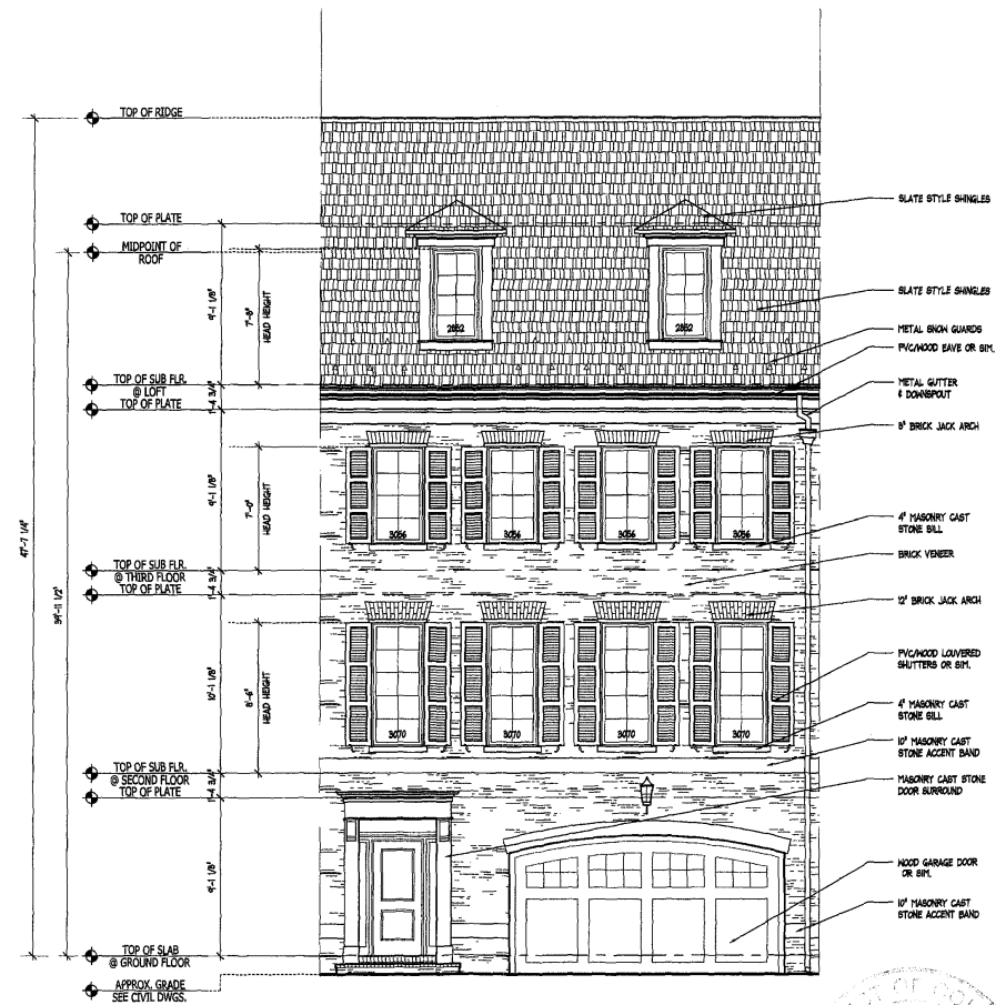
UNIT C FRONT ELEV. #2
