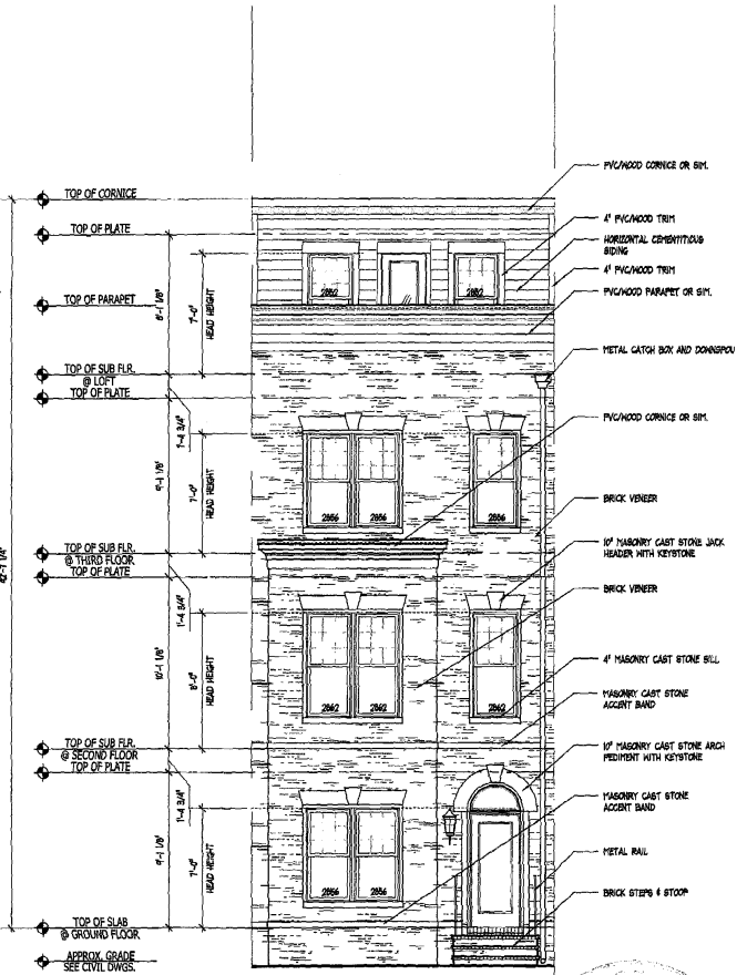
UNIT B FRONT ELEV. #3
