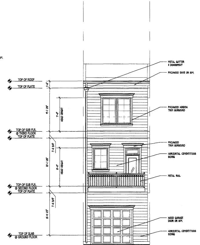
UNIT A REAR ELEV.
