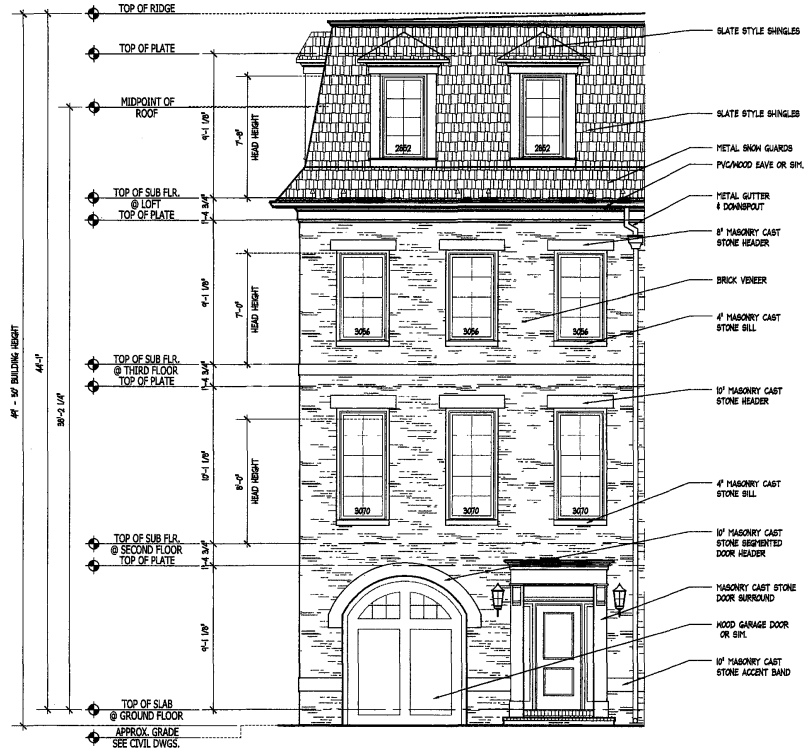
UNIT D FRONT ELEV. #1
