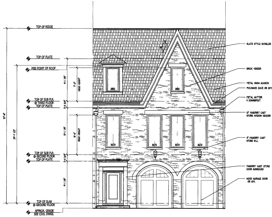
UNIT C1 FRONT ELEV. #3
