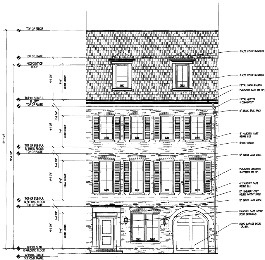
UNIT C FRONT ELEV. #3
