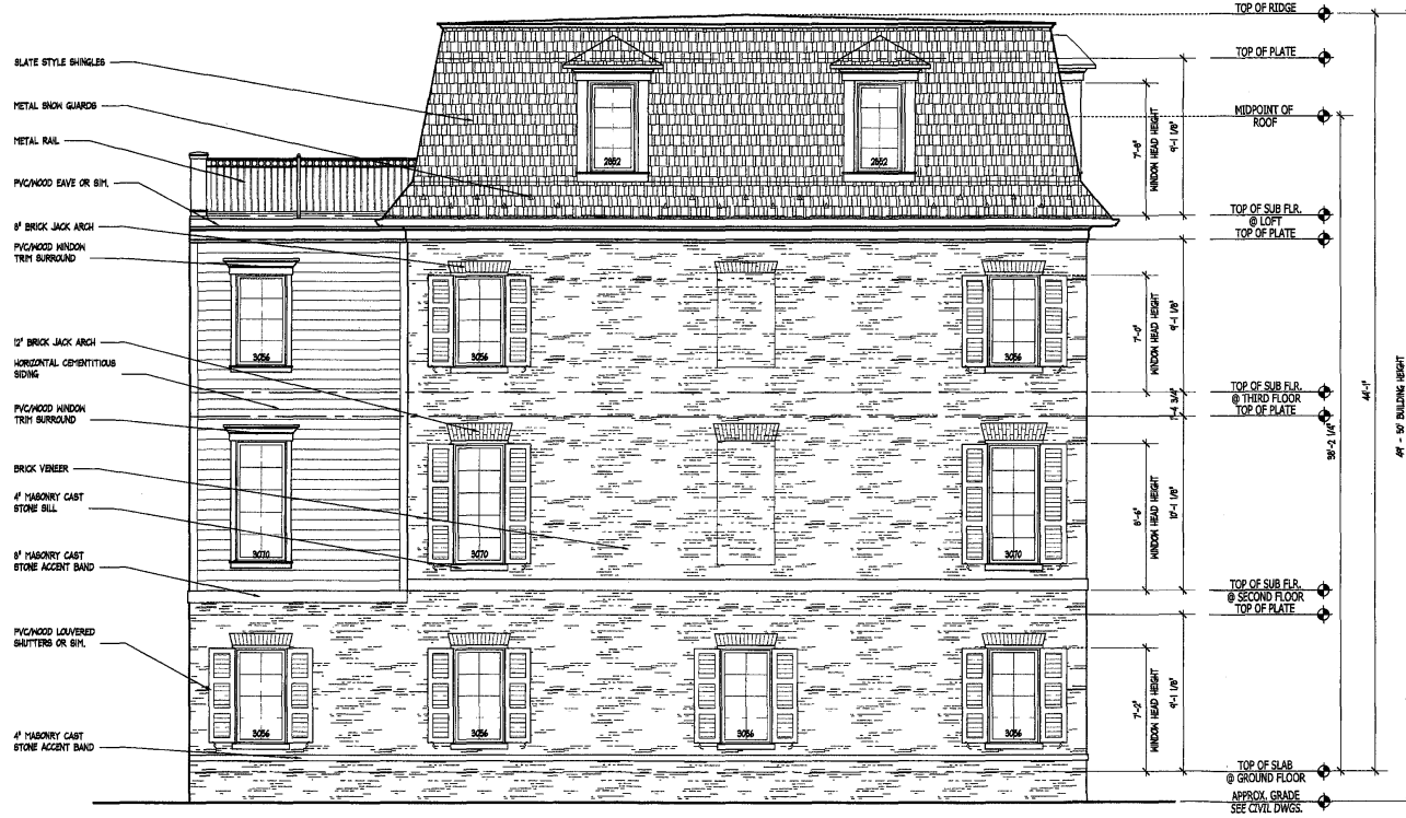
UNIT D FRONT ELEV. #2
