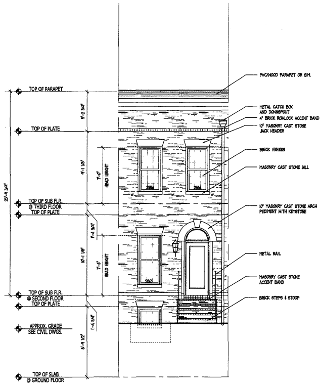
UNIT A FRONT ELEV. #1
