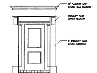
1 A-501 DOOR TYPE #1 Scale: 3/16"=1'-0"
