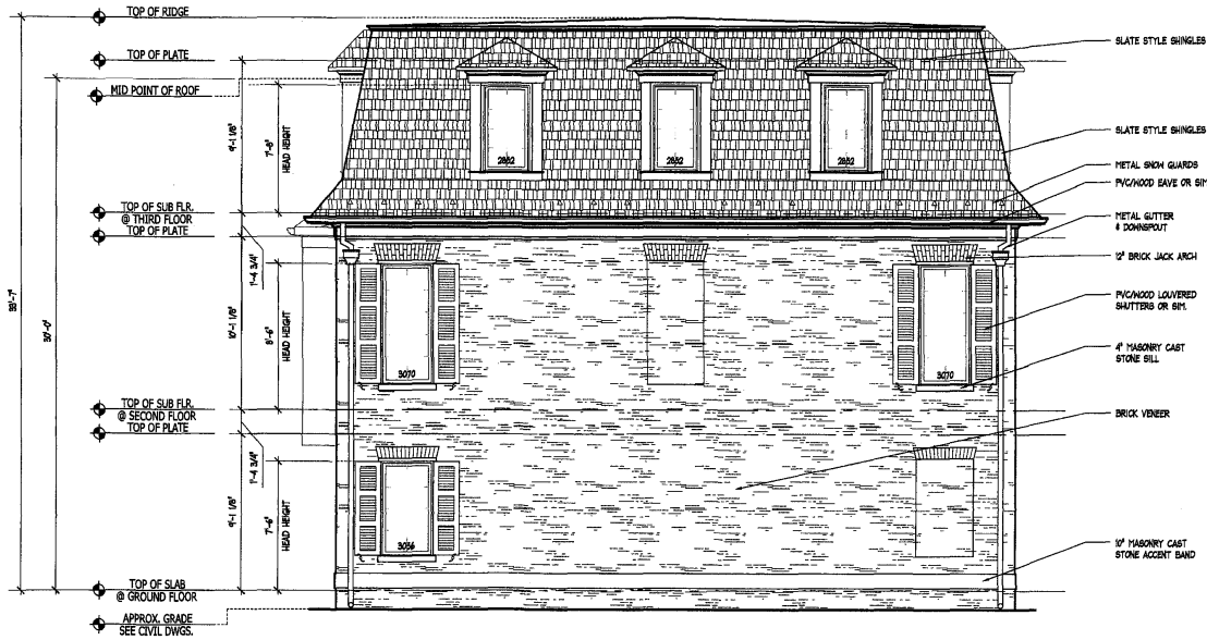
UNIT C1 FRONT ELEV. #1 & 4
