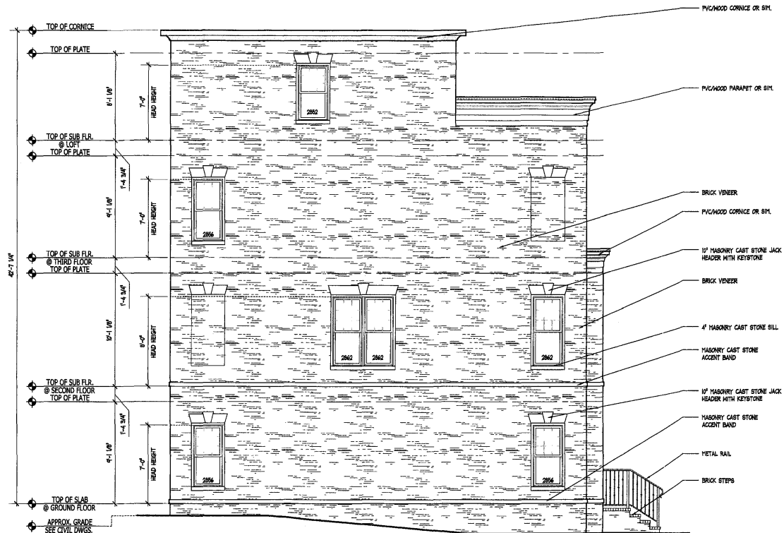
UNIT B SIDE ELEV. #3
