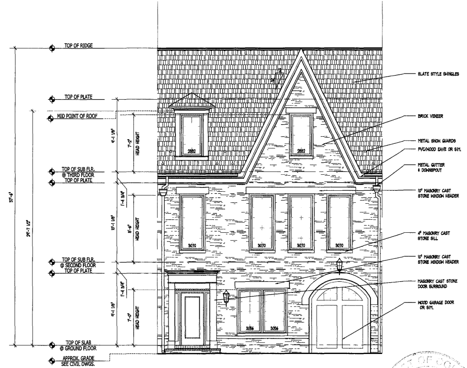
UNIT C1 FRONT ELEV. #2
