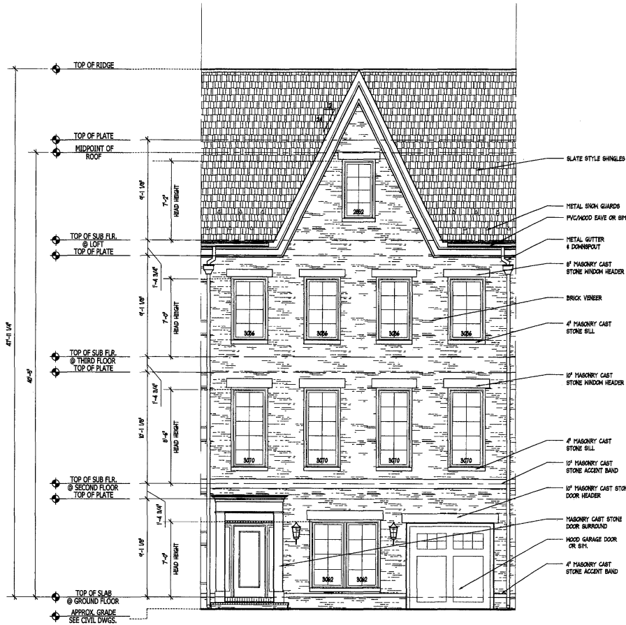
UNIT C FRONT ELEV. #5
