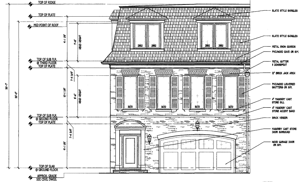
UNIT C1 FRONT ELEV. #4
