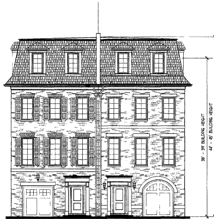
UNIT D ELEV. #2
