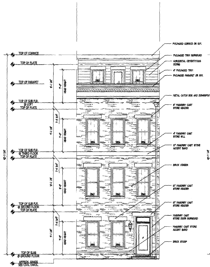
UNIT B FRONT ELEV. #1
