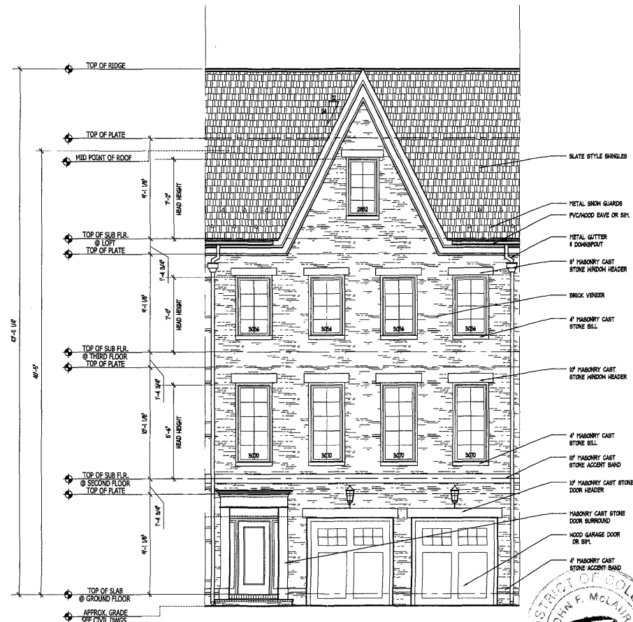
UNIT C FRONT ELEV. #4
