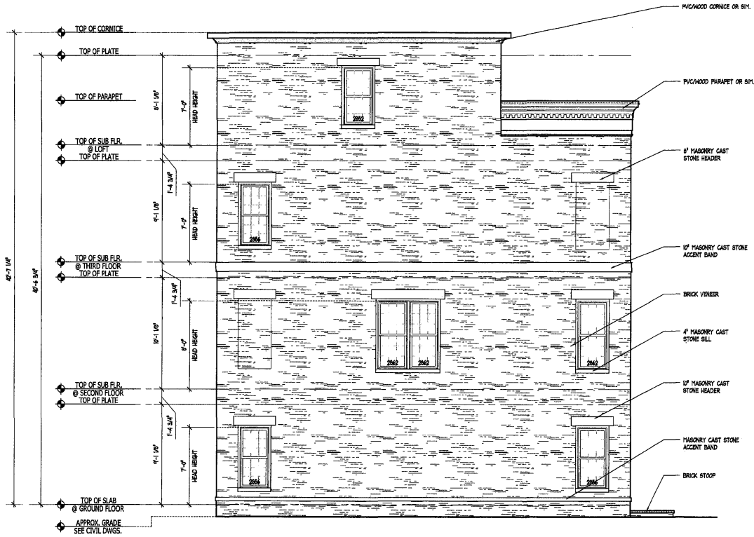
UNIT B SIDE ELEV. #1
