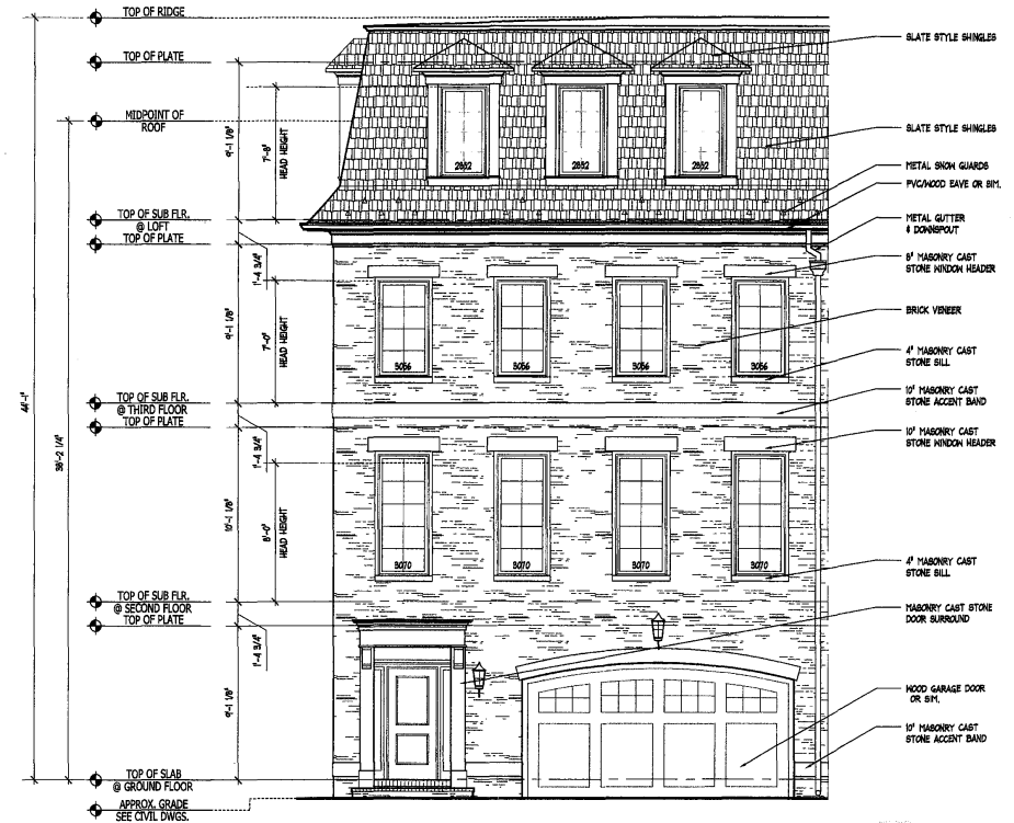
UNIT C FRONT ELEV. #6
