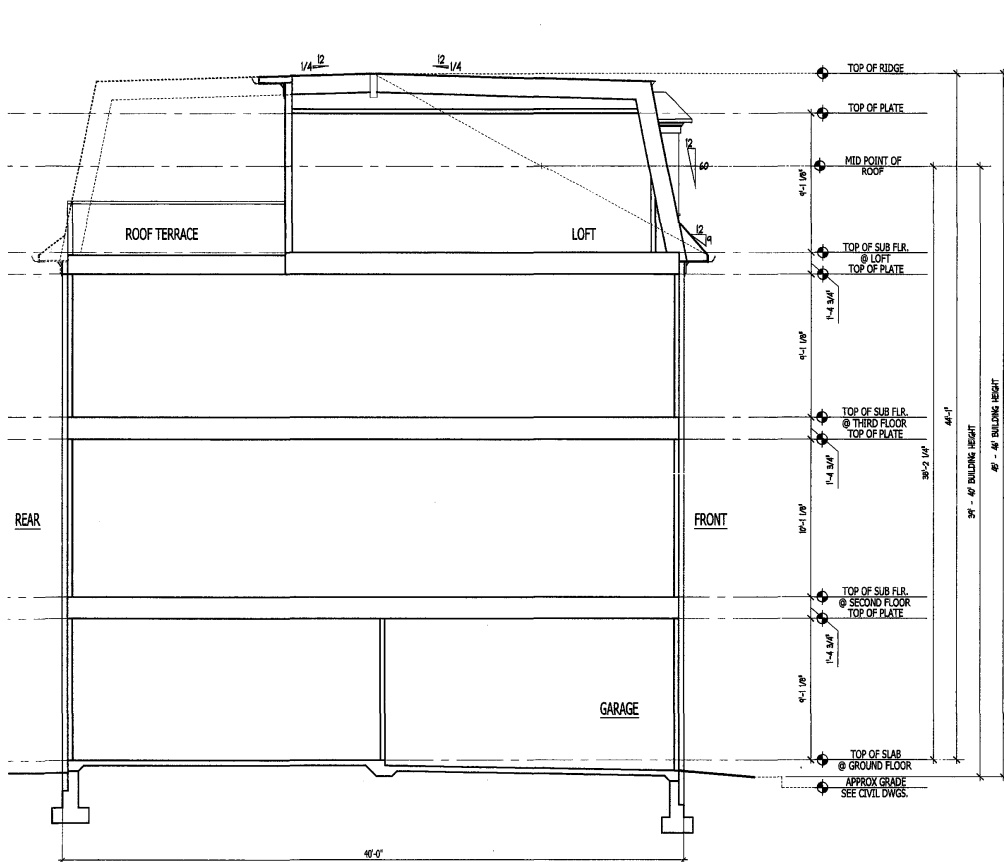
BUILDING SECTION - UNIT C - 4 STORY
