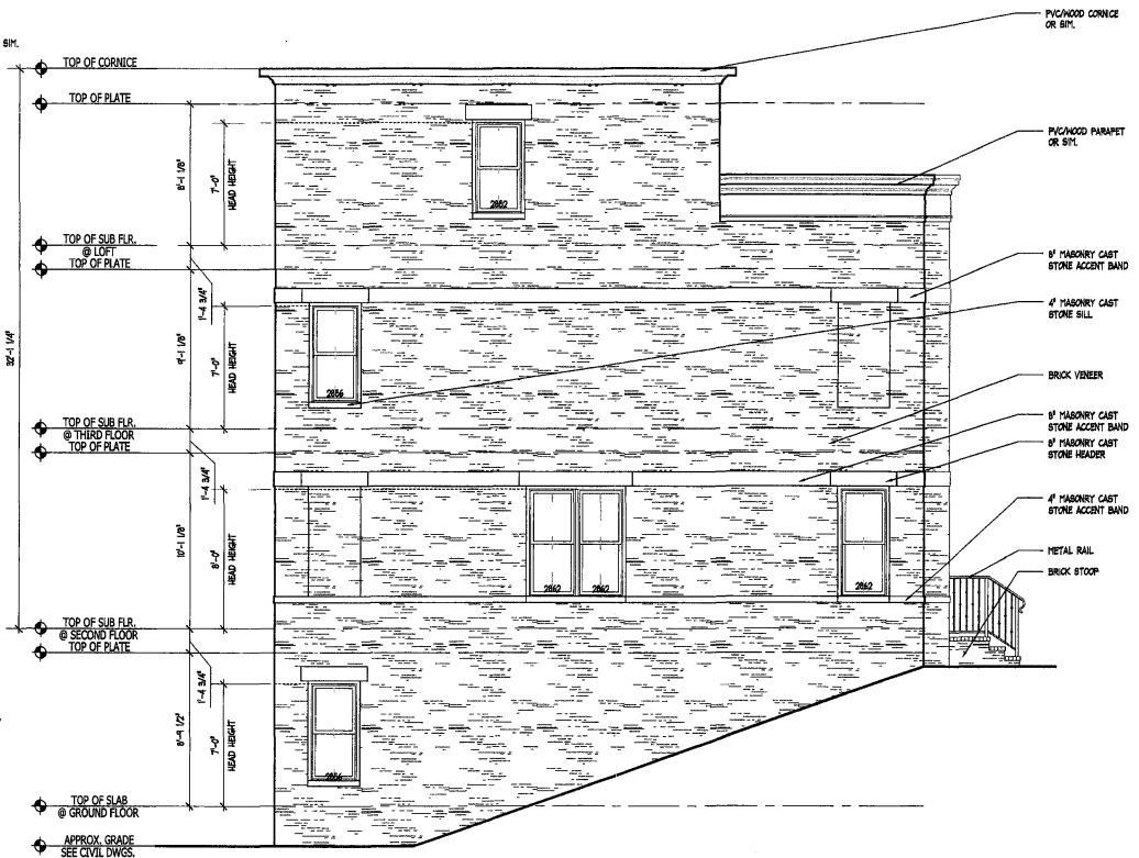
UNIT B1 SIDE ELEV. #2
