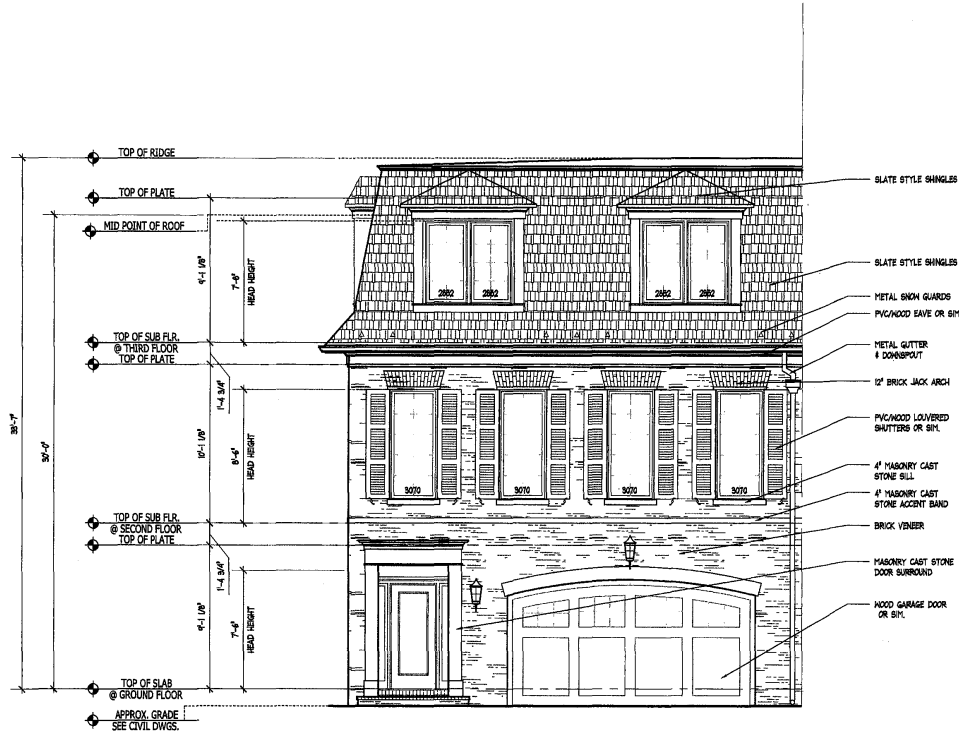
UNIT C1 FRONT ELEV. #1
