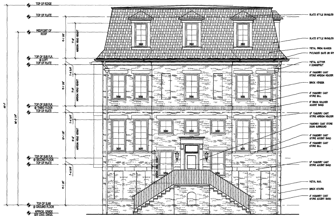
UNIT C FRONT ELEV. #1
