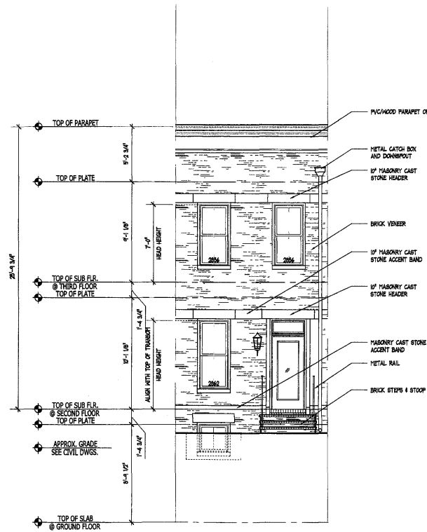
UNIT A FRONT ELEV. #2
