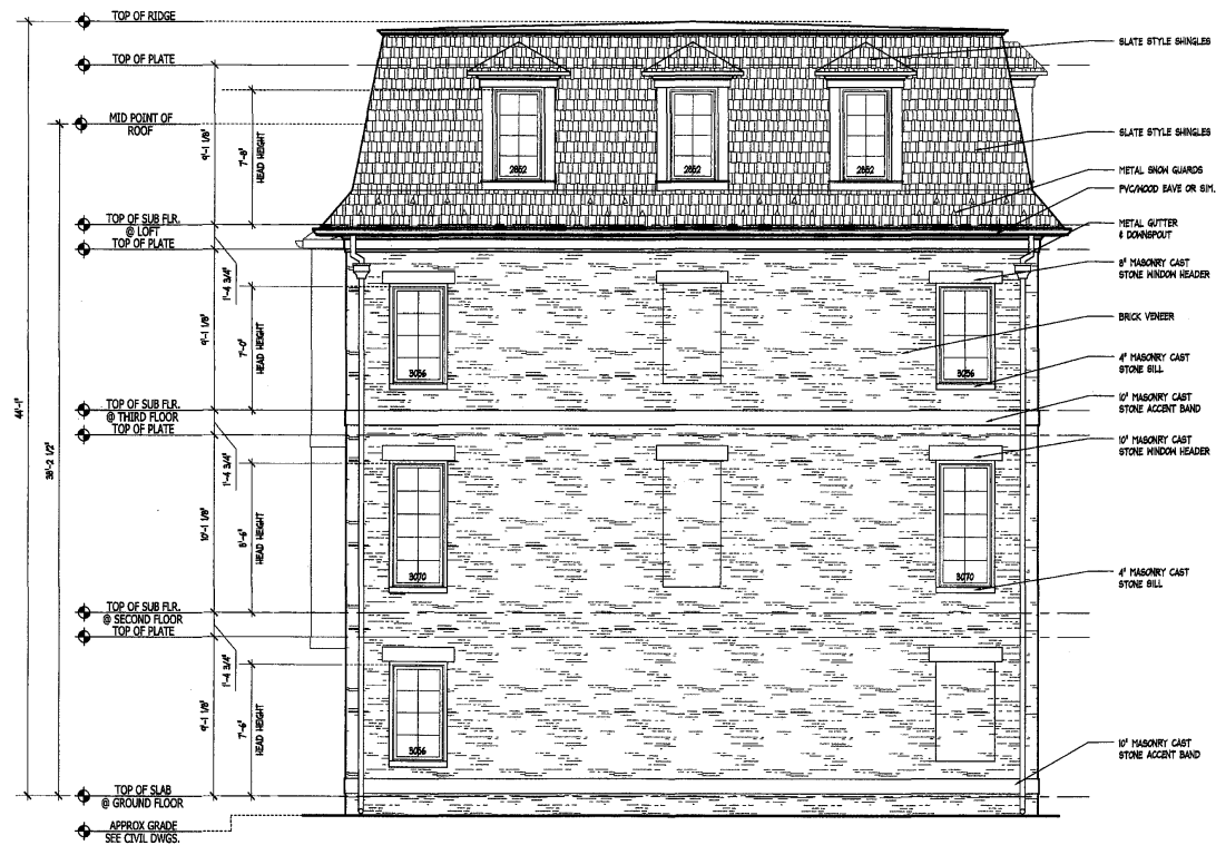
UNIT C FRONT ELEV. #6
