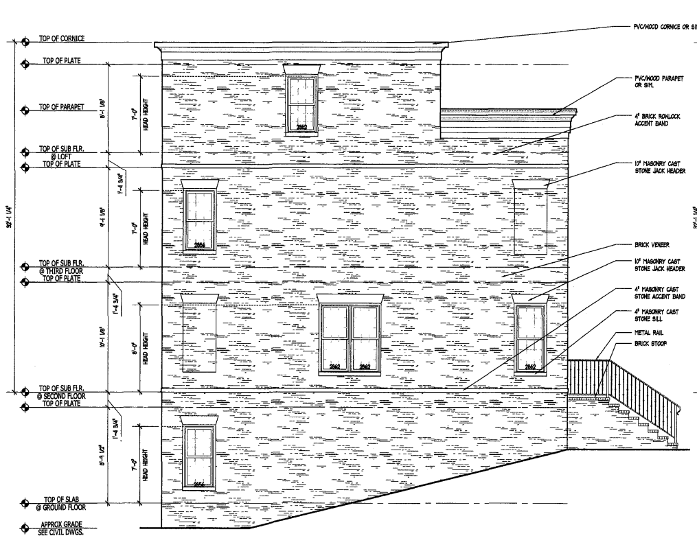
UNIT B1 SIDE ELEV. #1
