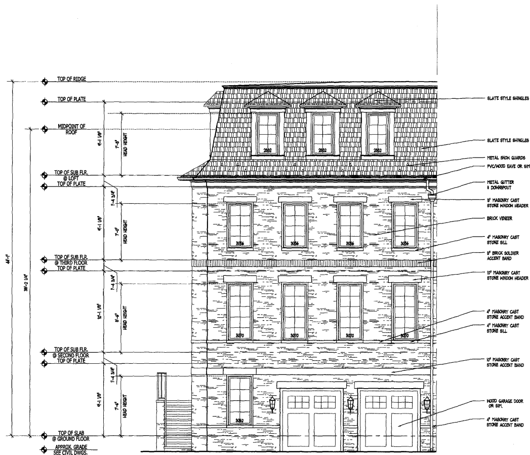
UNIT C FRONT ELEV. #1
