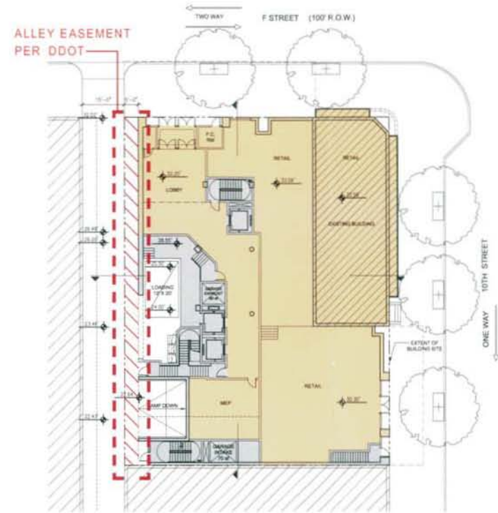
LEVEL 01 - PROPOSED
