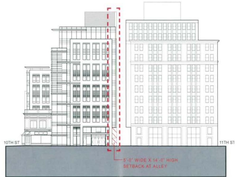
F STREET ELEVATION - PROPOSED
