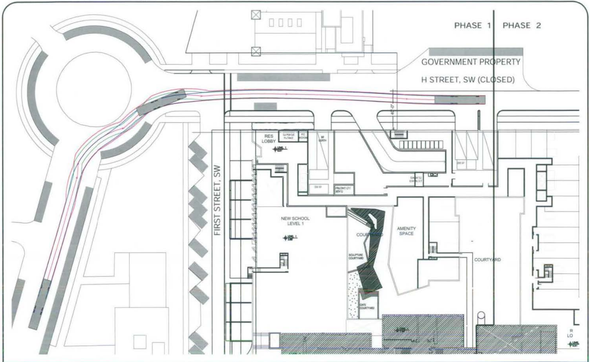
19 Figure 2-8 Swept Area Diagram - 52.5' Fire Truck - Inbound
