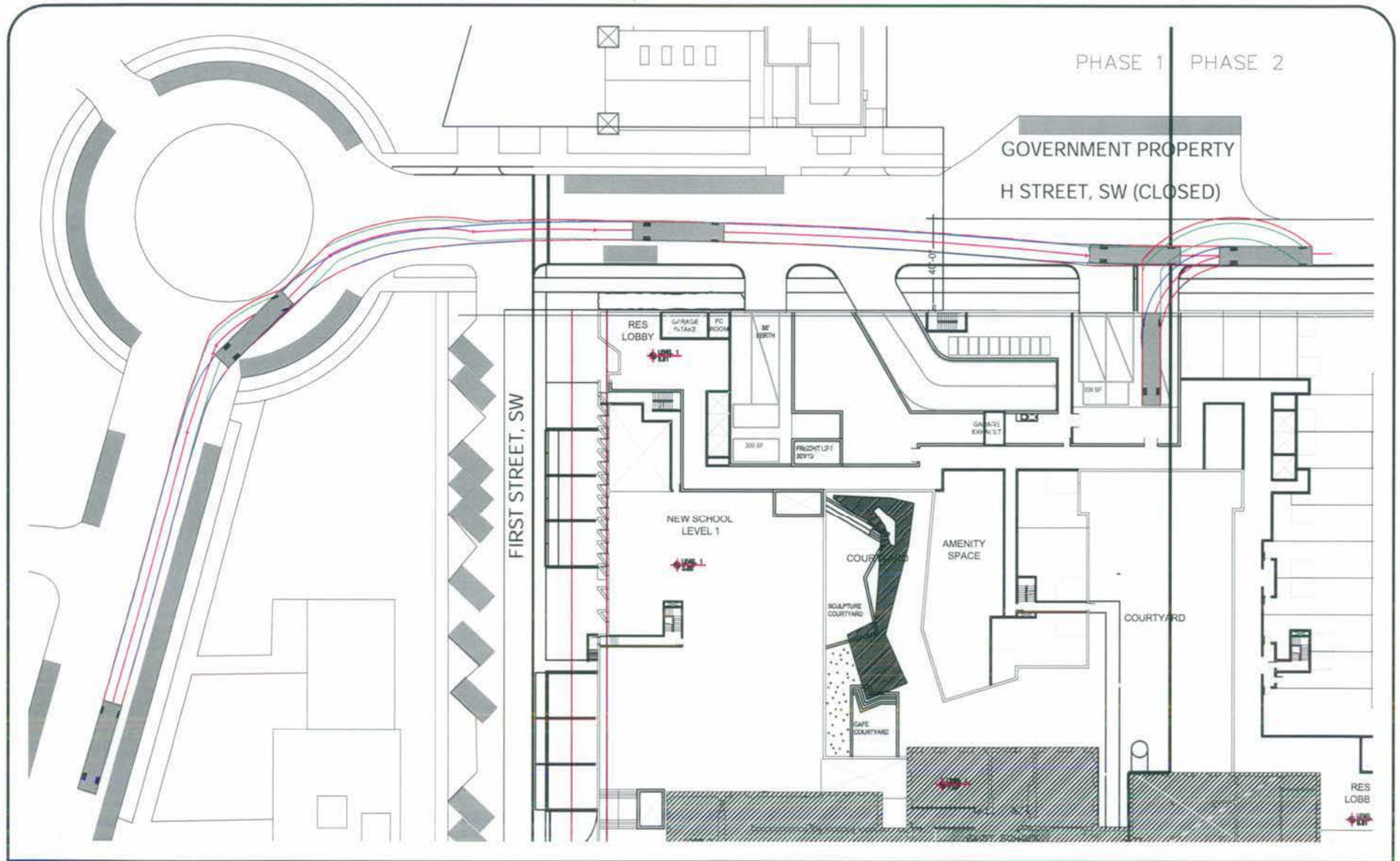
Figure 2-4 Swept Area Diagram - 40' (SU40) Single Unit Truck - Inbound
