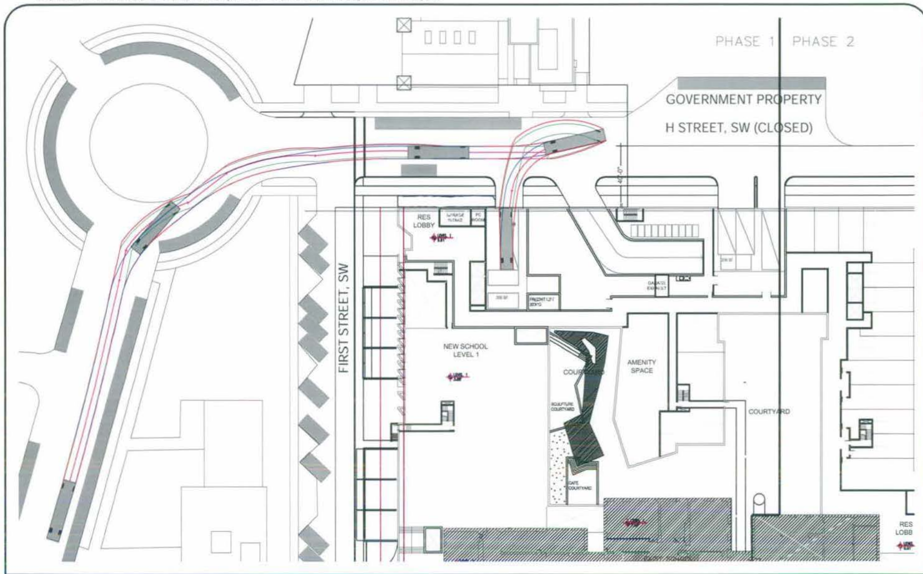
17 Figure 2-6 Swept Area Diagram - 40' (SU40) Single Unit Truck - Inbound
