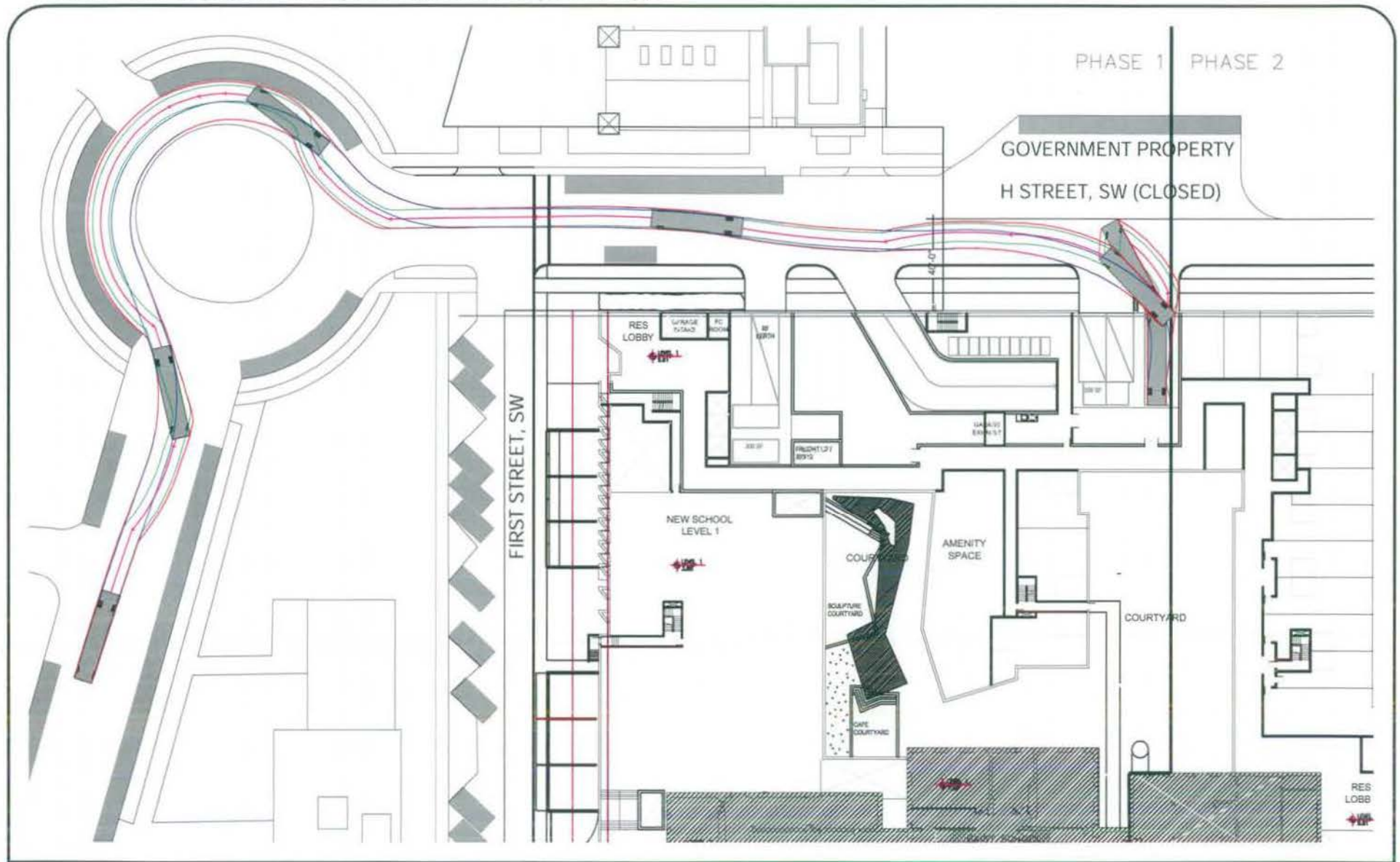
16 Figure 2-5 Swept Area Diagram - 40' (SU40) Single Unit Truck - Outbound
