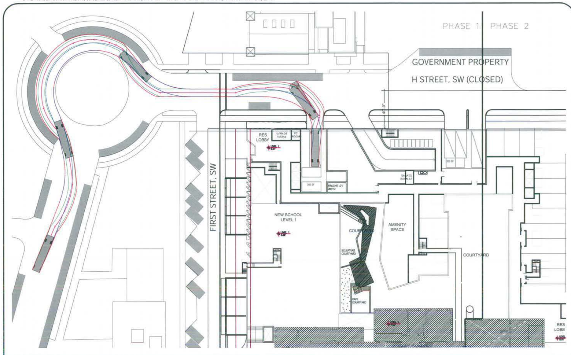
18 Figure 2-7 Swept Area Diagram - 40' (SU40) Single Unit Truck
