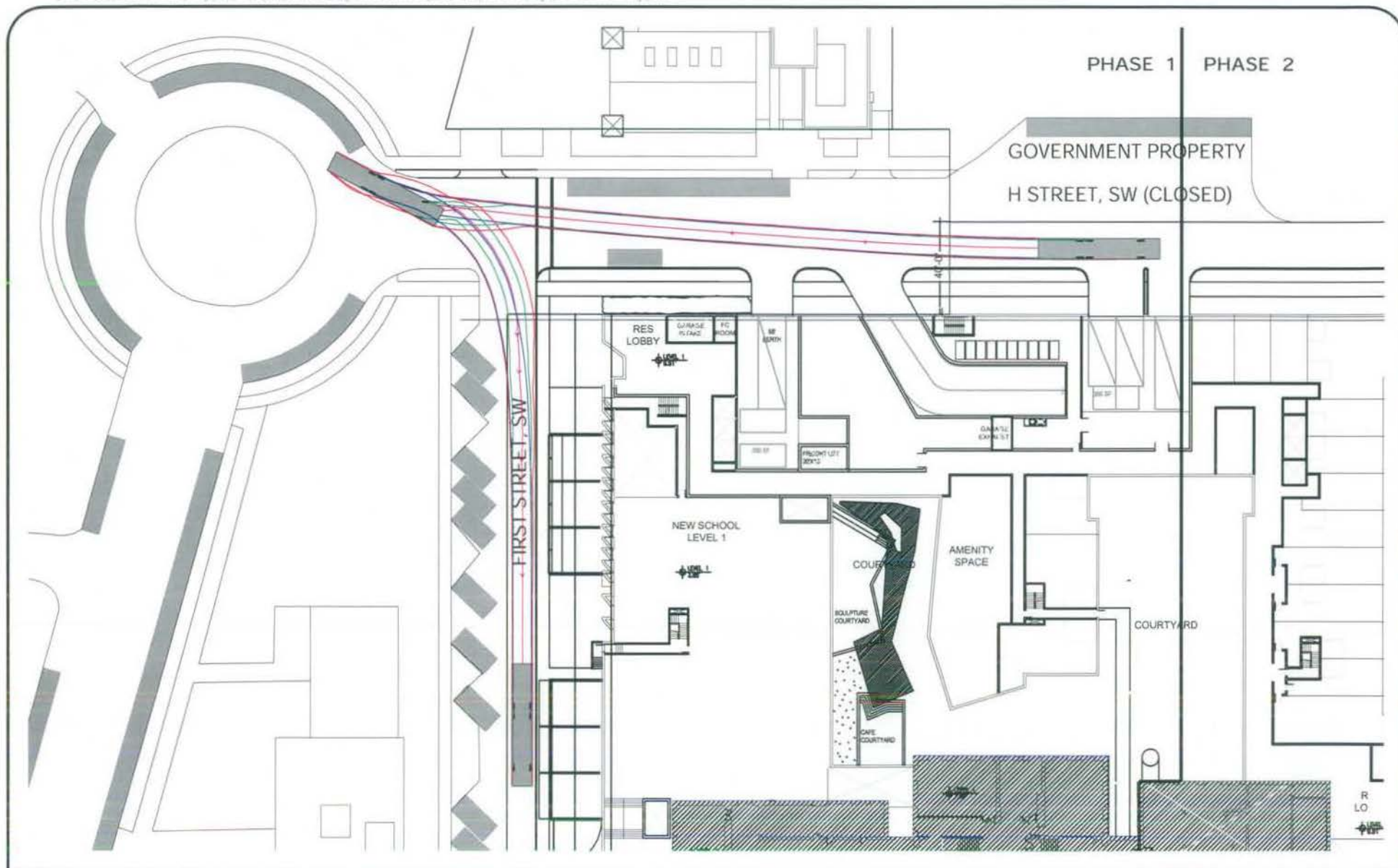
20 Figure 2-9 Swept Area Diagram - 52.5' Fire Truck - Outbound
