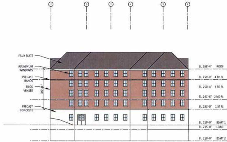
SOUTH ELEVATION
