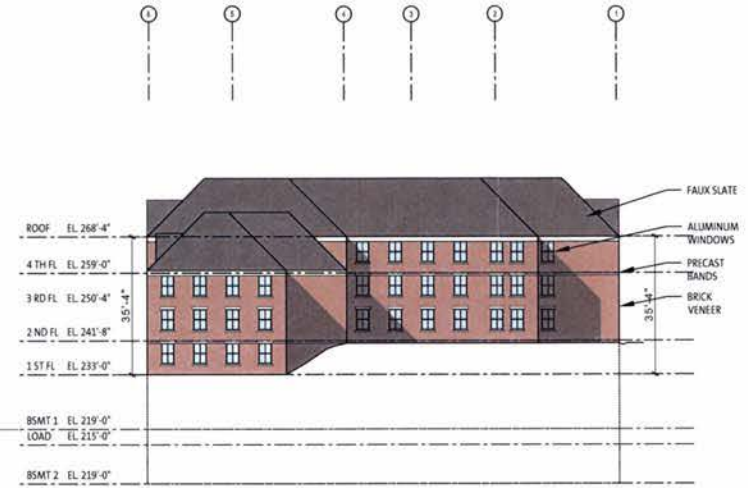
NORTH ELEVATION
