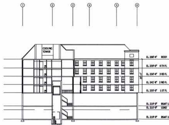
TRANSVERSE SECTION FACING NORTH
