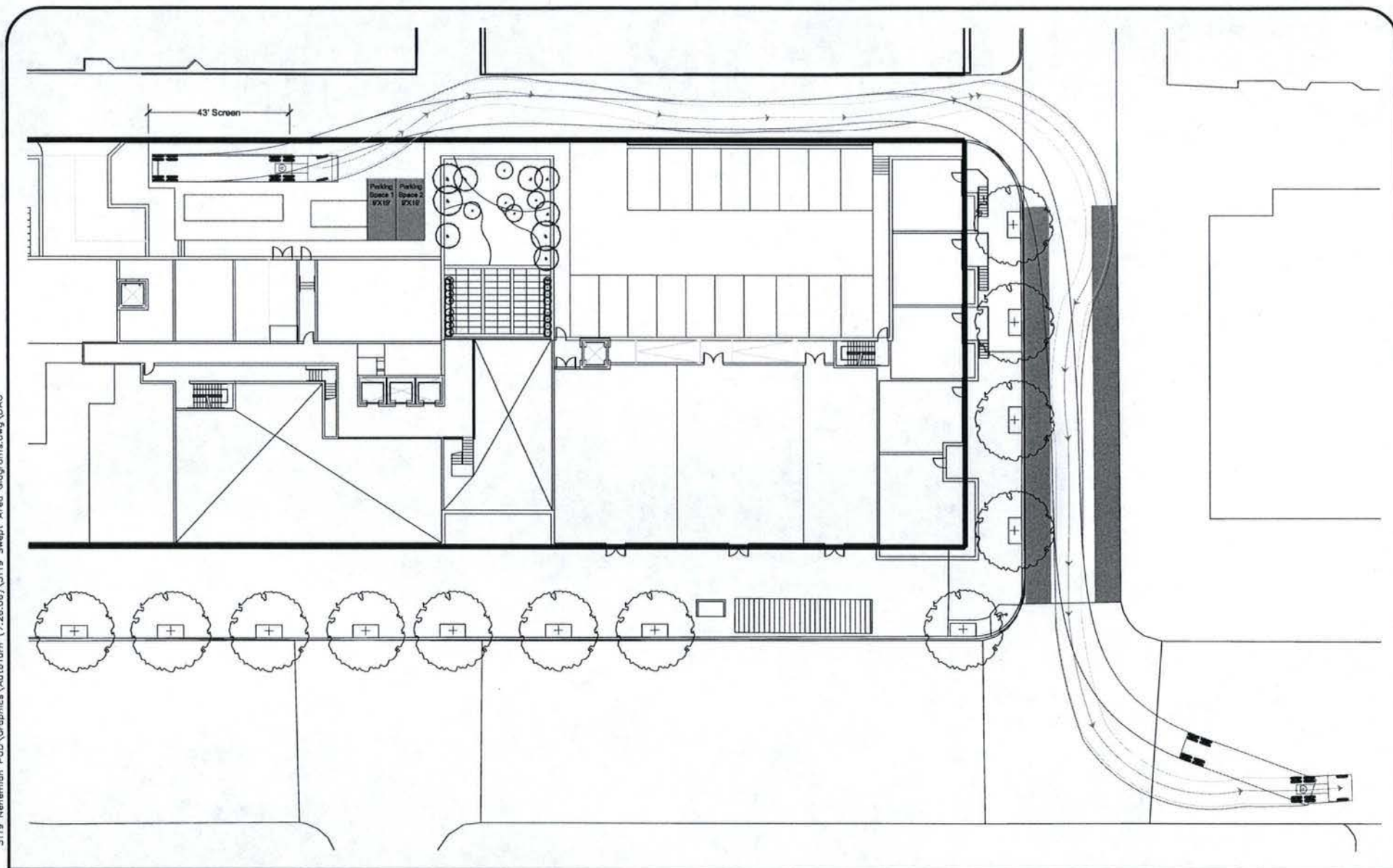
Diagram 1 WB50 Semitrailer Exiting From Loading Area To 14th Street.
