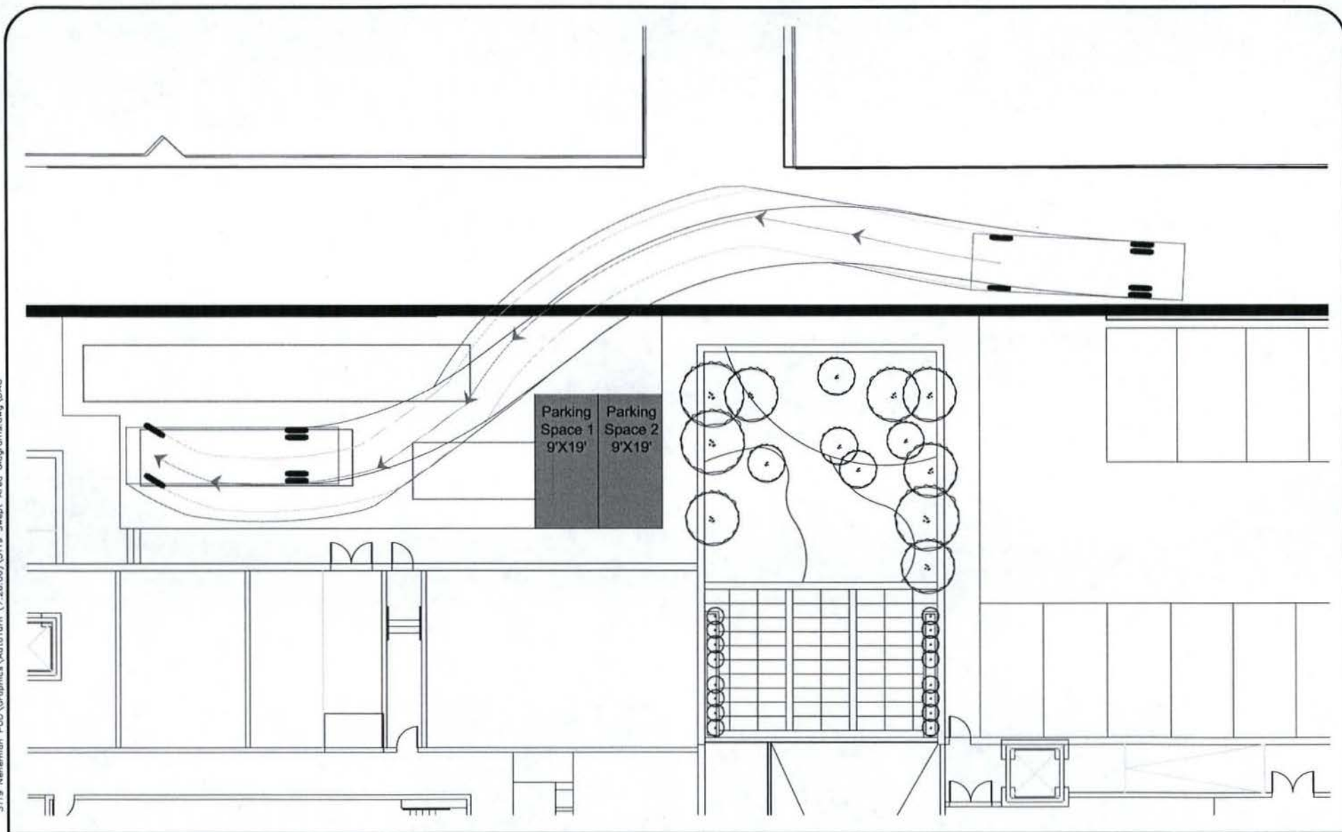
Figure 30' Single Unit Docking With Two Flex Parking Spaces
