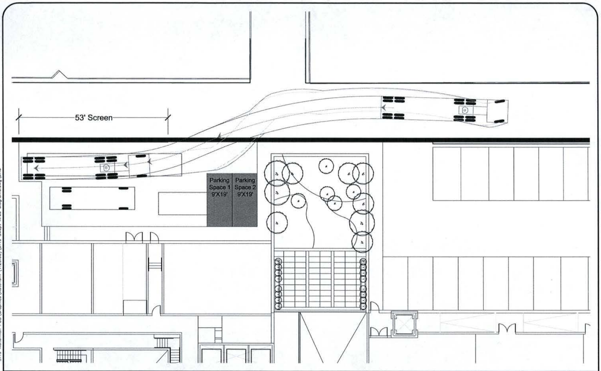
Figure WB40 Docking With Two Flex Parking Spaces
