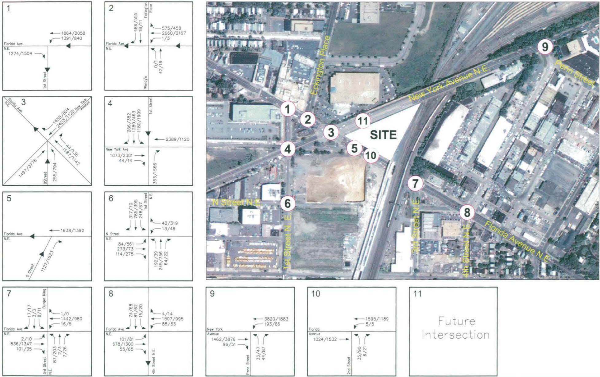
37 Figure 3-6 Background Future Peak Hour Traffic Forecasts with New York Avenue/Florida Avenue Circle
