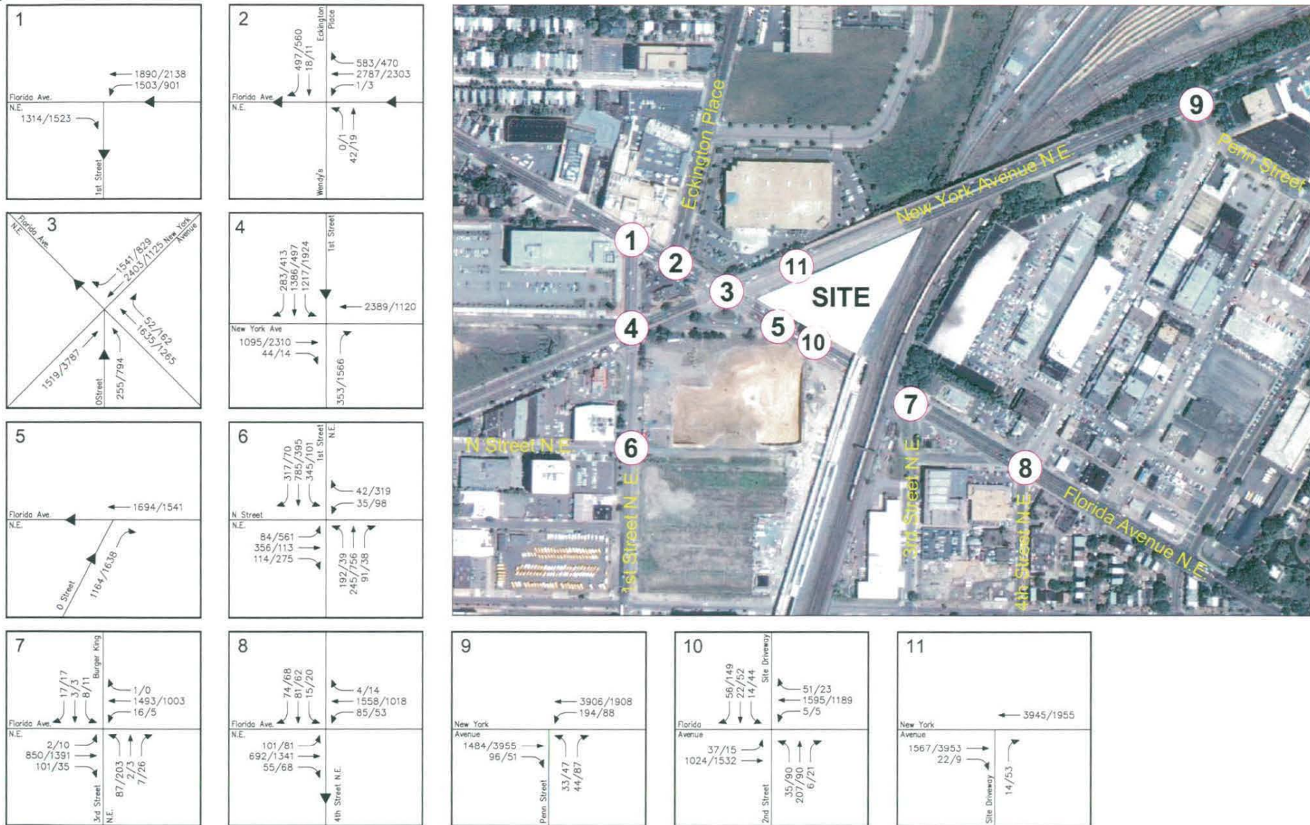
Figure 3-10 Total Future Traffic Forecasts with New York Avenue/Florida Avenue
