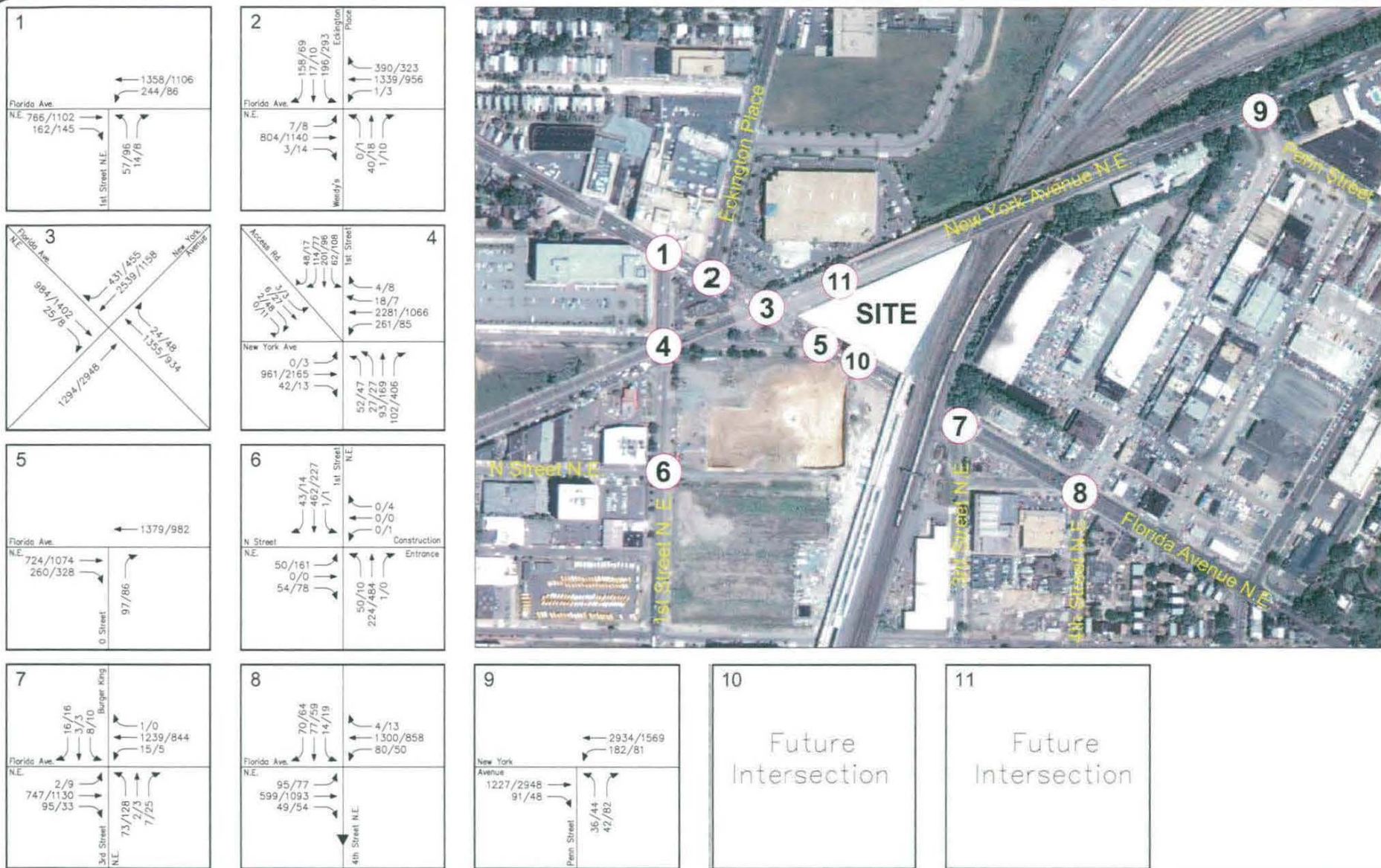
Figure 2-7 Existing Peak Hour Vehicular Traffic Counts
