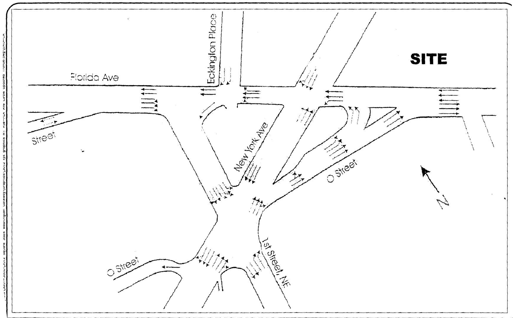
14 Figure 2-2 Planned New York Avenue/Florida Avenue Circle
