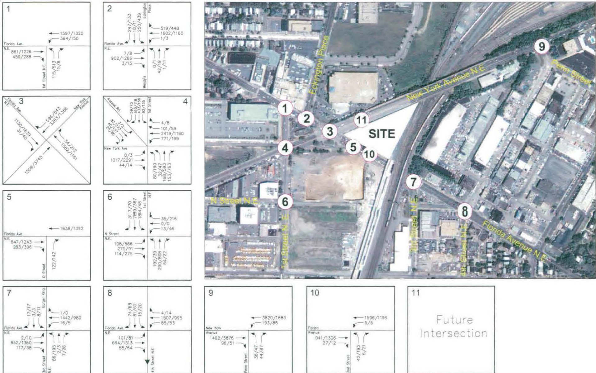
Figure 3-5 Background Future Peak Hour Traffic Forecasts
