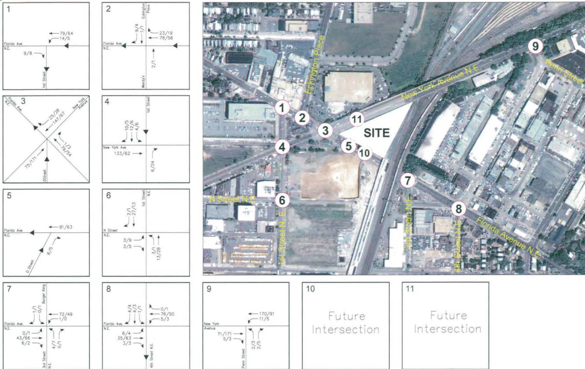
Figure 3-4 Background Growth with New York Avenue/Florida Avenue Circle
