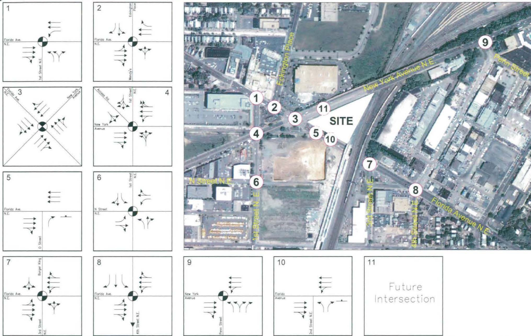
Figure 2-3 Background Lane Use and Traffic Control
