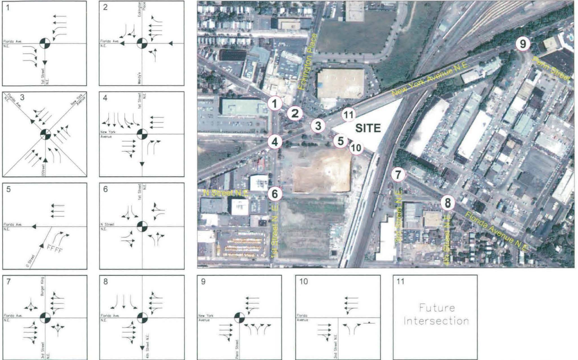
Figure 2-4 Background Lane Use with New York Avenue/Florida Avenue Circle
