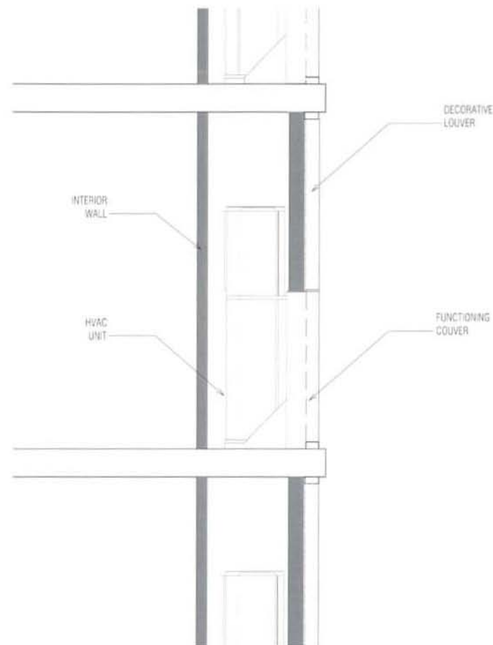
Section with Heat Pump Unit and Louver
