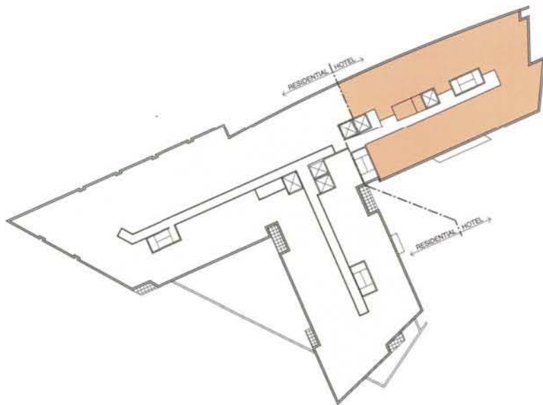
1 3RD-10TH(-11TH HOTEL) FLOOR PLAN
