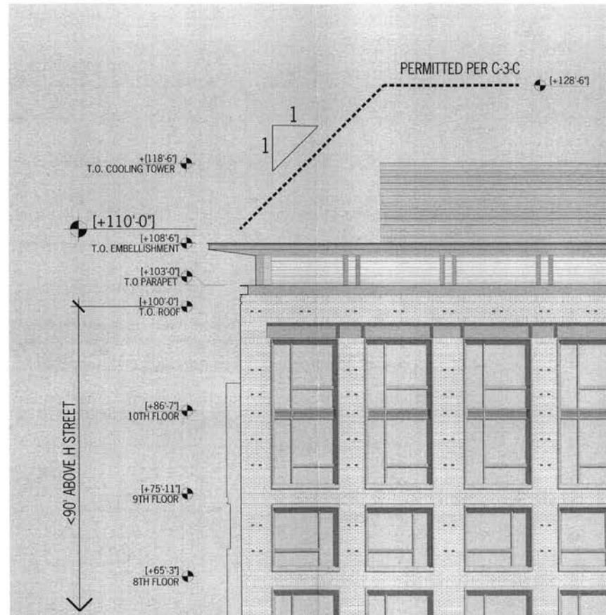
Capitol Place tower elevation detail
