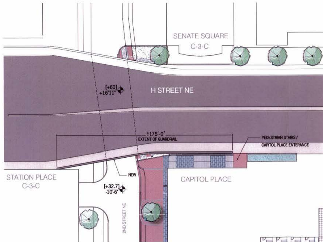
Site plan at H Street overpass
