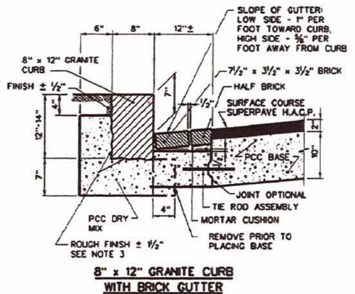
Granite Curb and Brick Gutter DC DOT Standard
