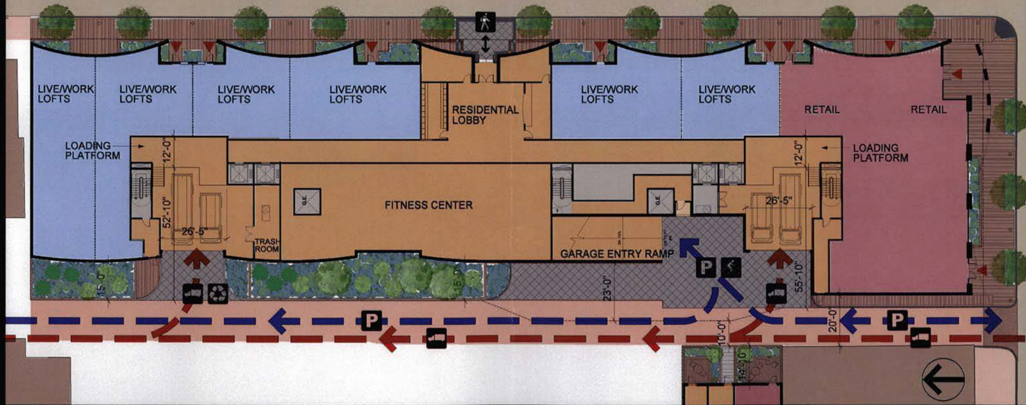
Parcel A - Ground Floor Plan
