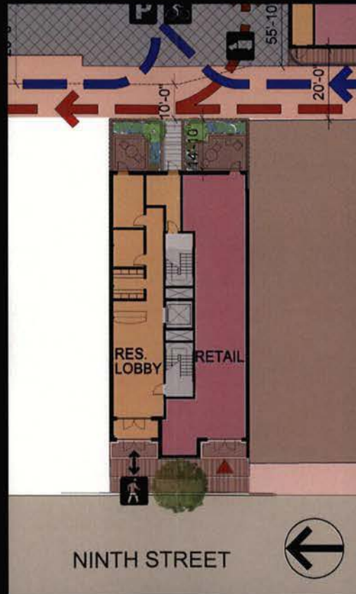
Parcel D - Ground Floor Plan
