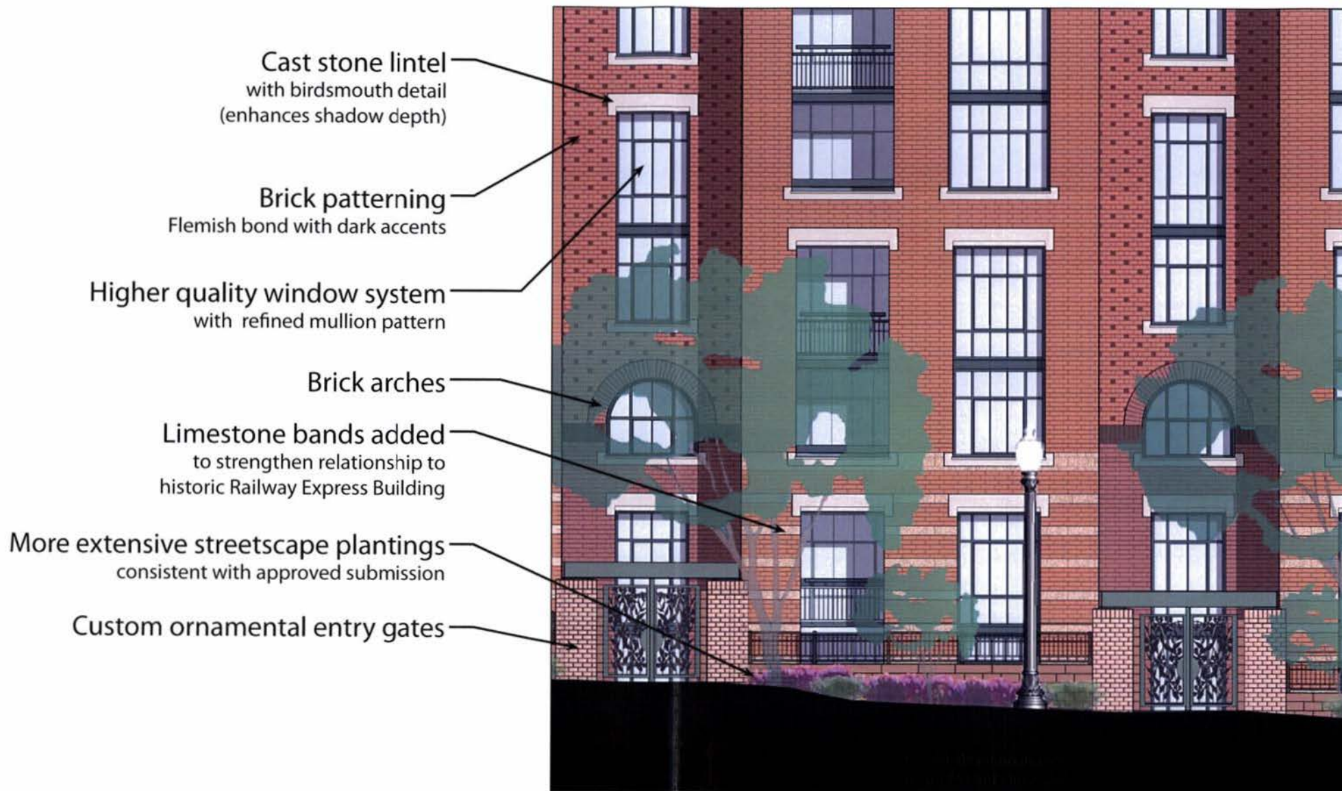
Enlarged elevation at base Second Street elevation
