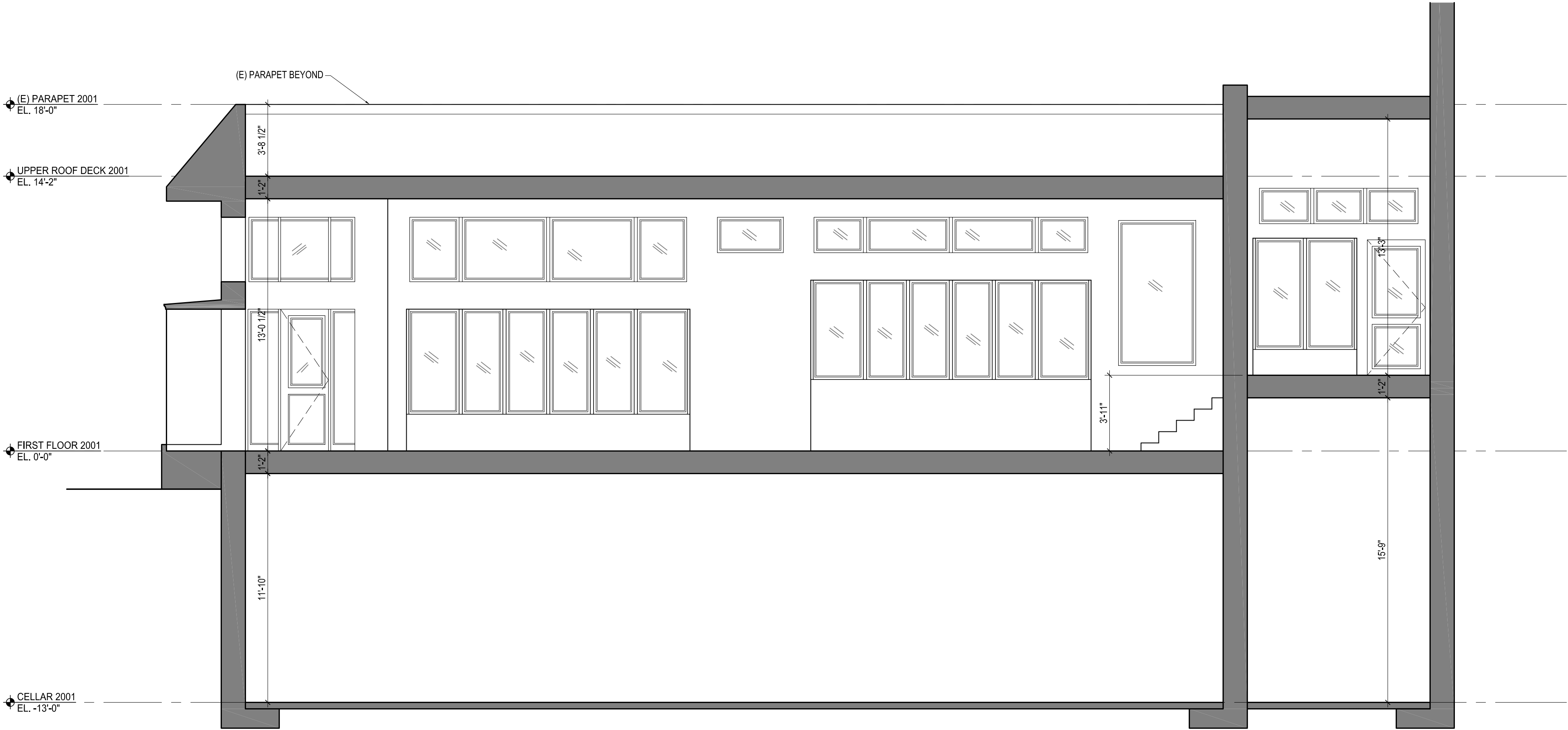
1 | WEST SECTION
