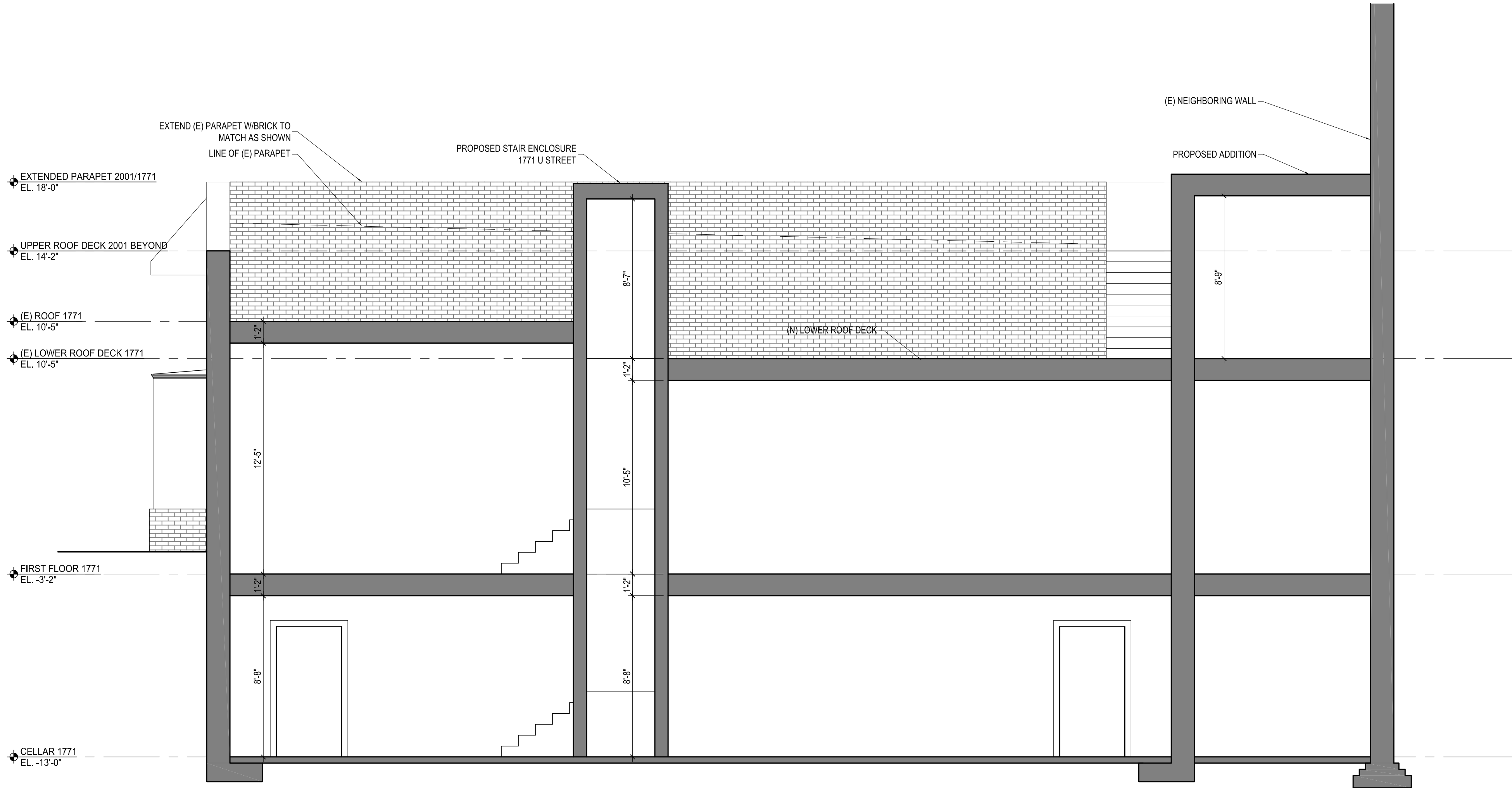
2 | WEST SECTION
