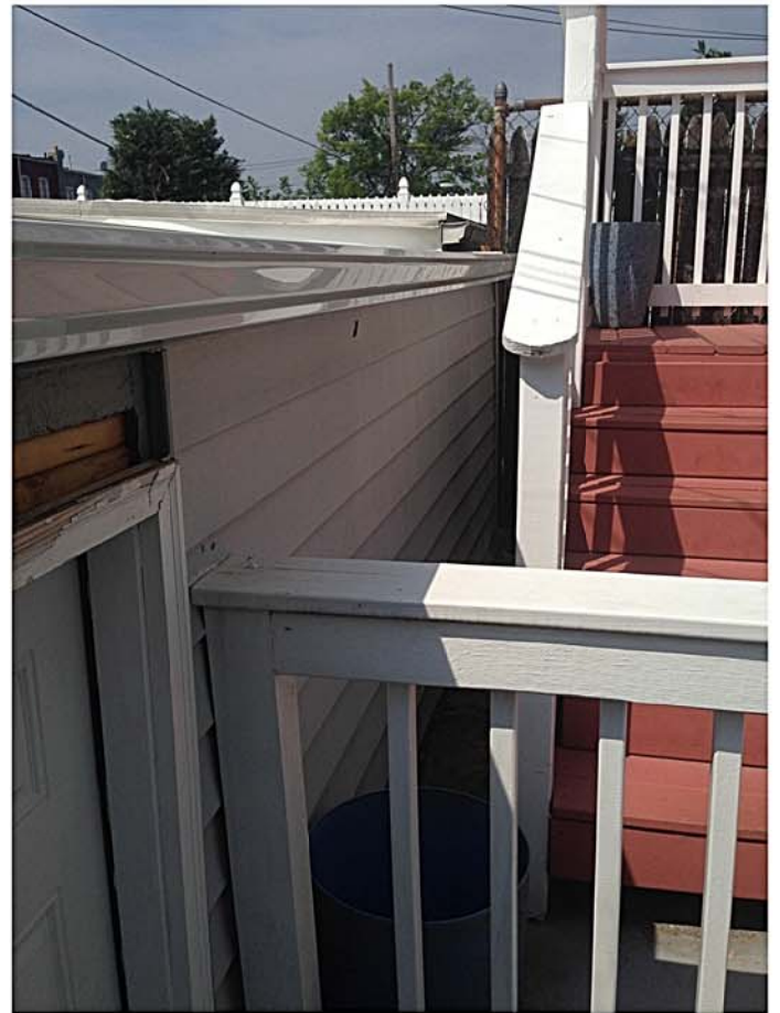
EXISTING STAIR CONNECTION W/ GARAGE
